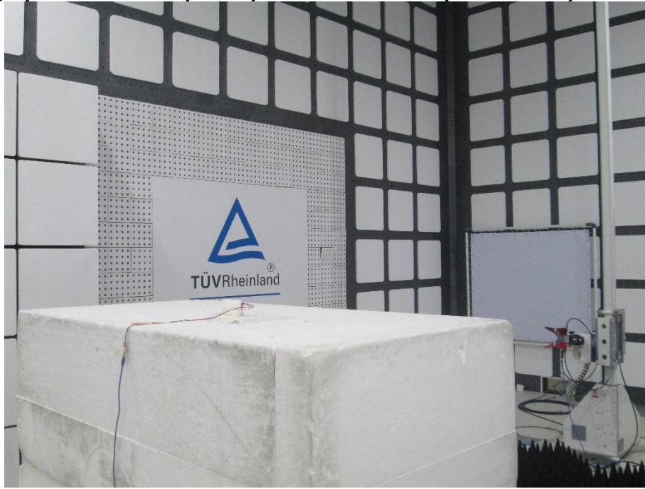
Photograph 38: Test Setup for Spurious Emissions (Back View 4)
