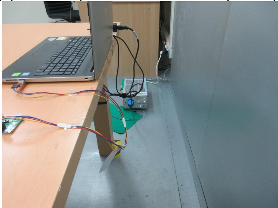
Photograph 24: Test Setup for Mains Conducted Emissions (Back View)
