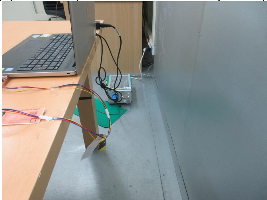
Photograph 32: Test Setup for Mains Conducted Emissions (Back View)
