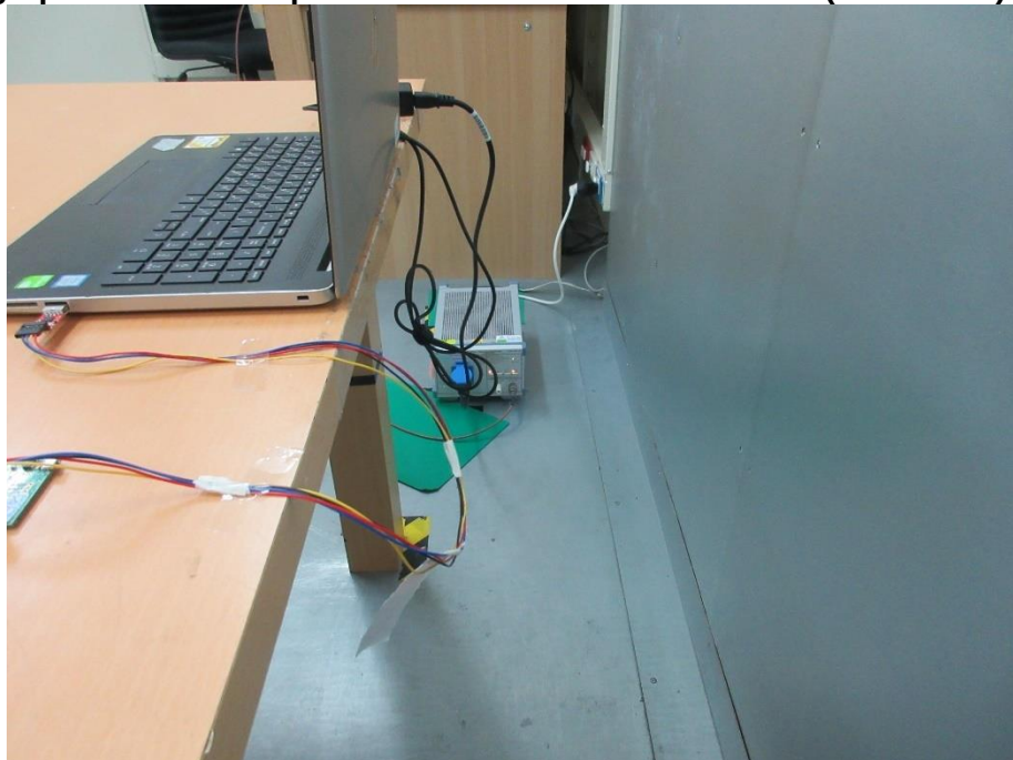
Photograph 40: Test Setup for Mains Conducted Emissions (Back View)
