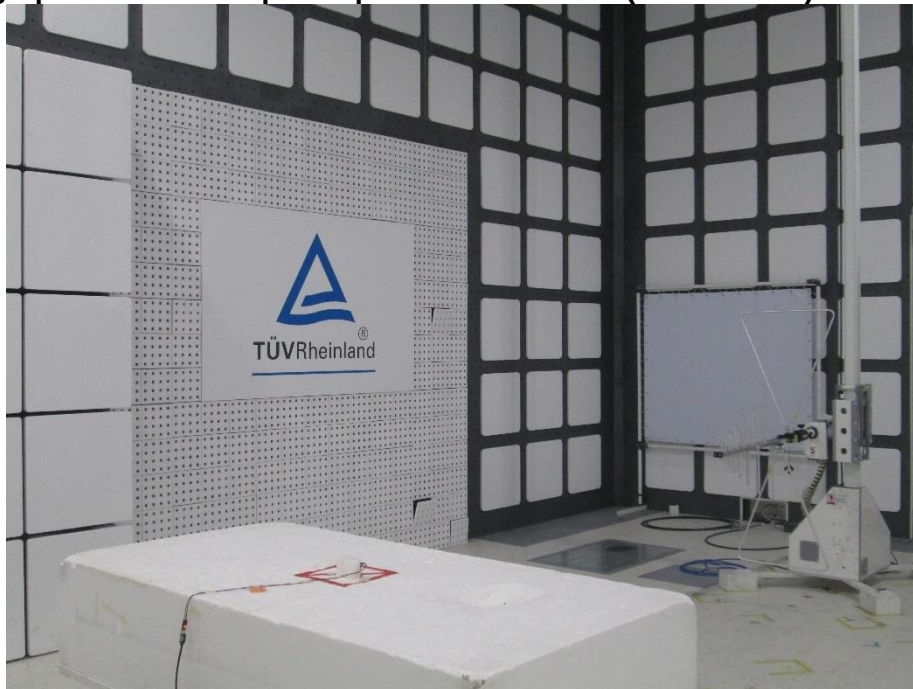
Photograph 36: Test Setup for Spurious Emissions (Back View 2)
