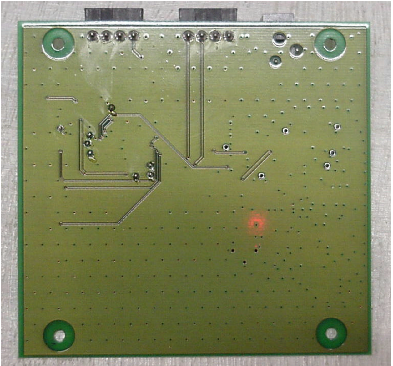
Photo 5. Internal Board Solder Side
