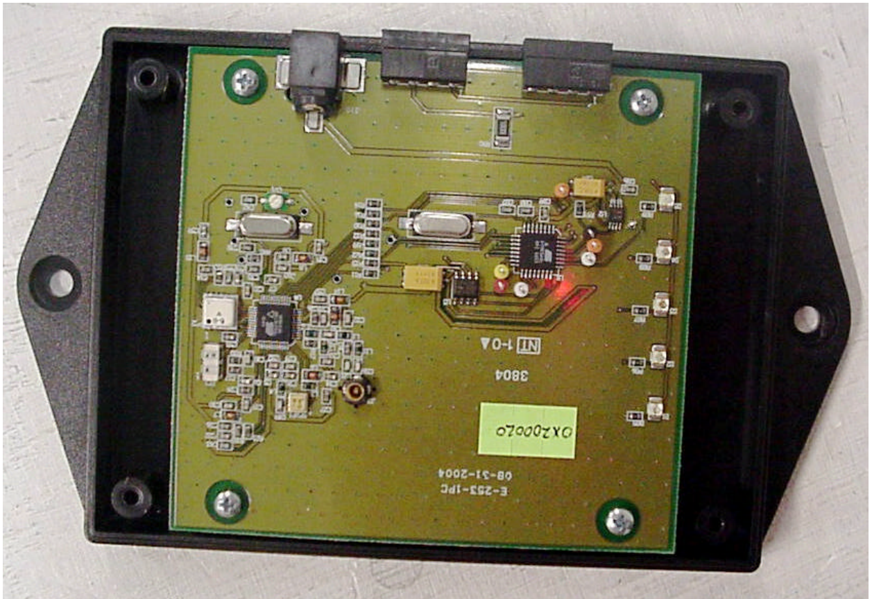
Photo 4. Internal Board Component Side
