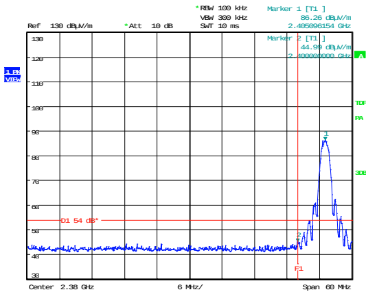
Band-Edge Compliance – Lower Edge Variant #2 Channel: 11
