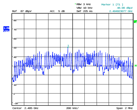
Power Spectral Density Variant #2 Channel: 11
