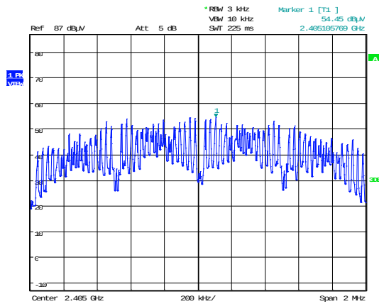
Power Spectral Density Variant #1 Channel: 11
