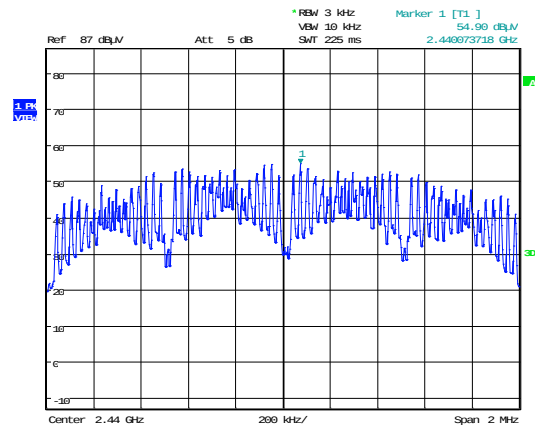
Power Spectral Density Variant #1 Channel: 18
