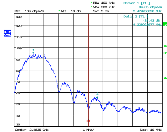
Band-Edge Compliance – Upper Edge Variant #1 – 100 kHz BW Channel: 26
