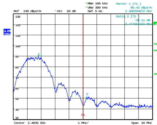
Band-Edge Compliance – Upper Edge Variant #2 – 100 kHz BW Channel: 26
