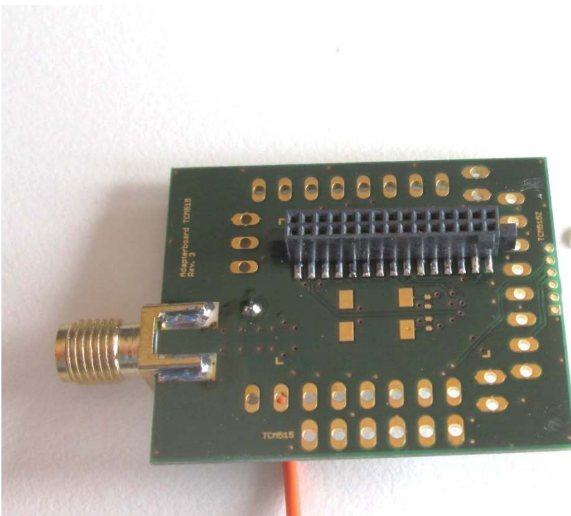
Photo A2-2: EUT Variant #1 – Bottom view
