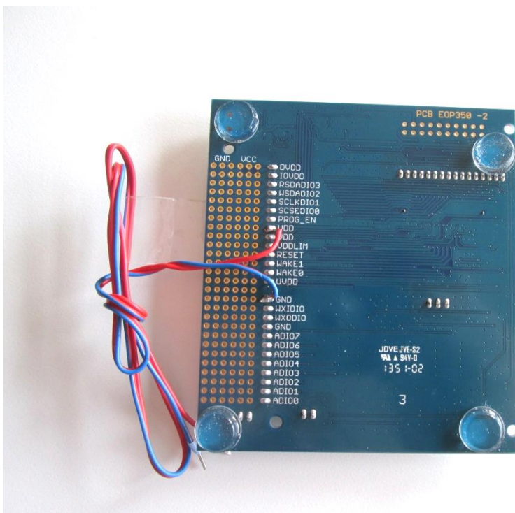
Photo A3-2: Eval-Board EOP350 – Bottom view
