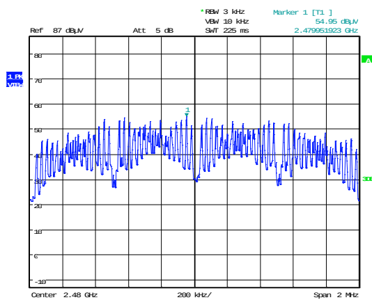
Power Spectral Density Variant #1 Channel: 26
