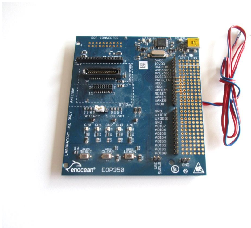
Photo A3-1: Eval-Board EOP350 – Top view
