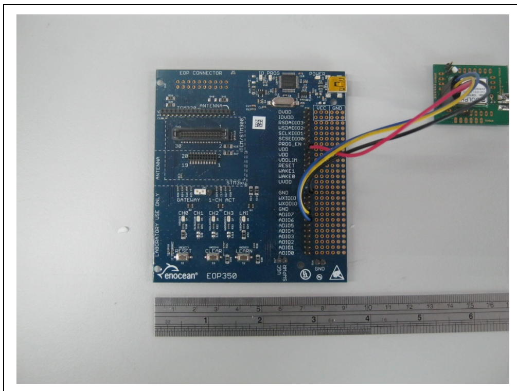
Photograph A3-2: Eval Board EOP 350, top view
