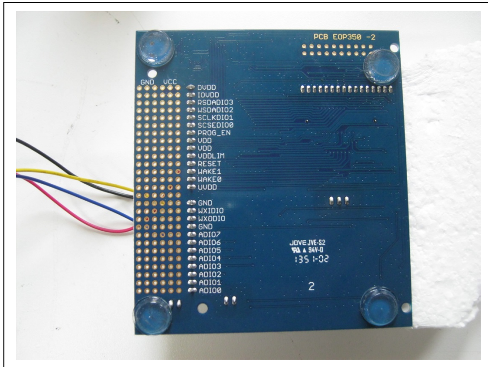
Photograph A3-3: Eval Board EOP 350, bottom view
