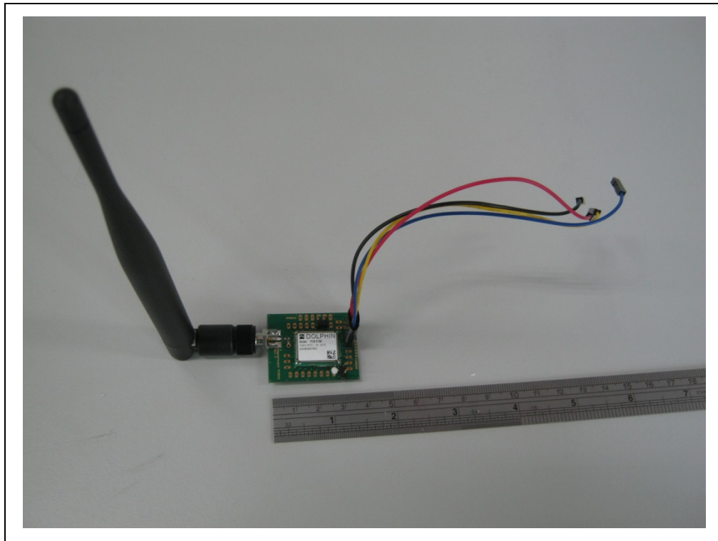
Photograph A2-1: EUT#1 top, with antenna
