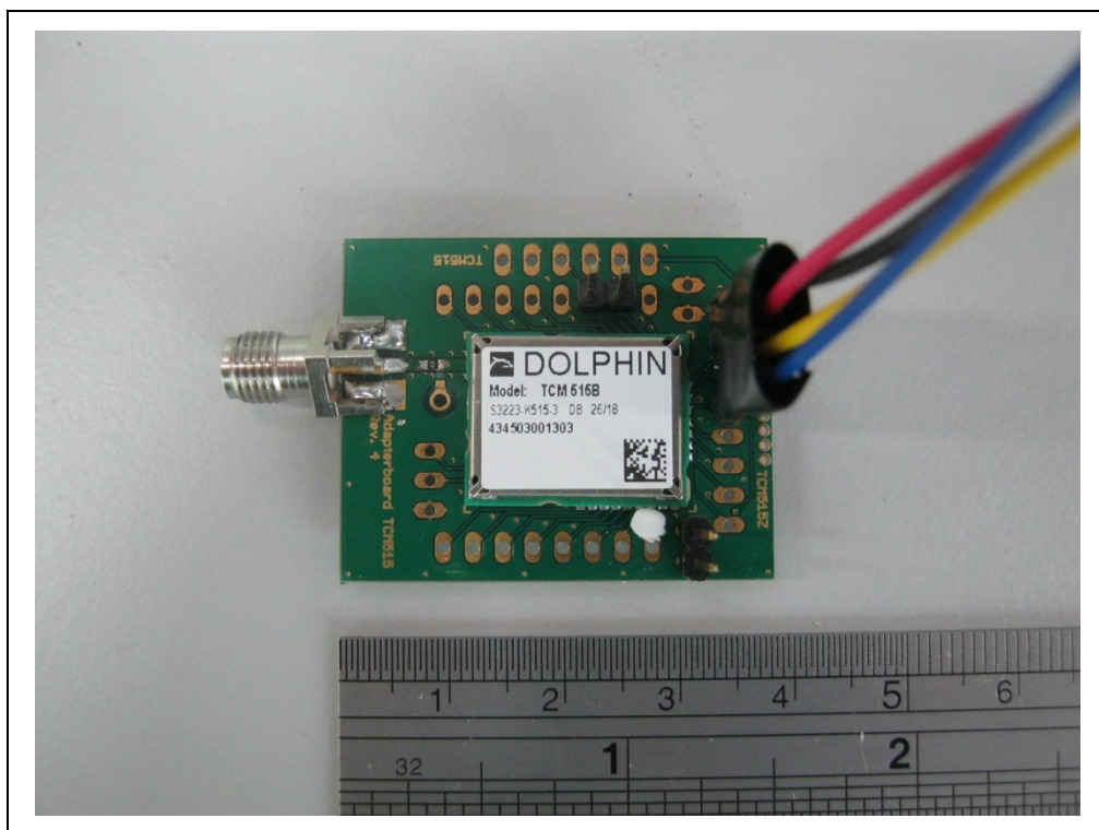
Photograph A2-2: EUT#1 top, without antenna
