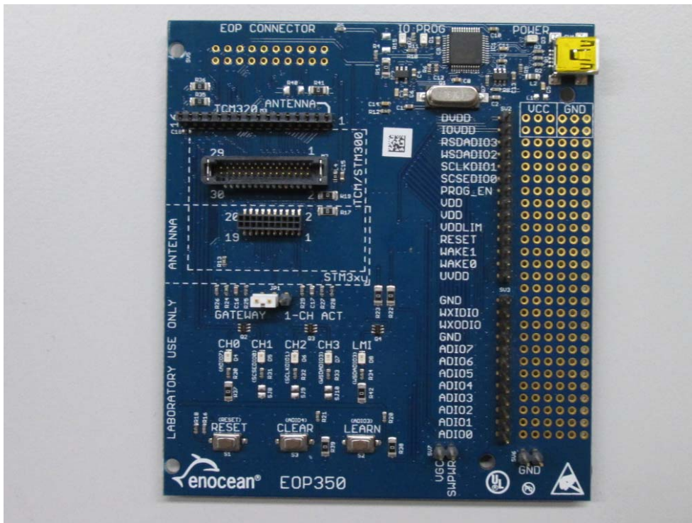
Photo A3-1: Eval-Board EOP350 – Top view
