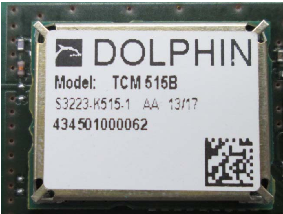
Photo A2-10: EUT Variant #3 – Label
