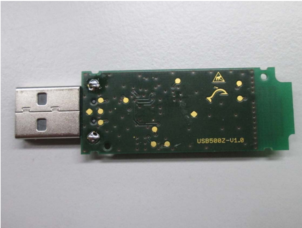
Photo A2-9: EUT Variant #3 – Bottom view
