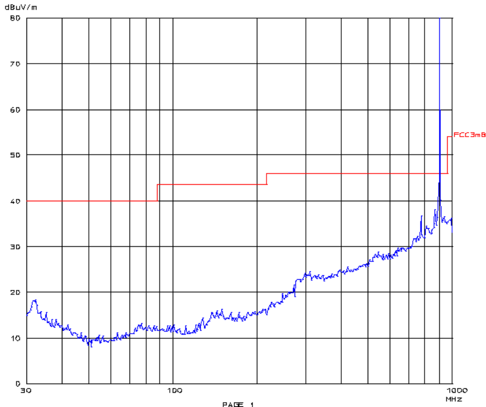
Plot 6.7.3-1: EUT STM 333U, sample 1, pre-scan plot d = 3m (30 MHz to 1 GHz)
