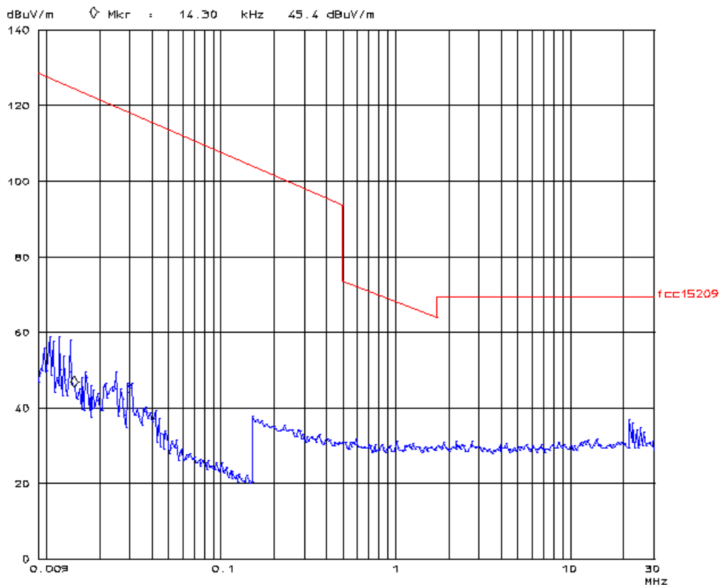
Plot 6.7.2.1: EUT STM 333U, sample 1, Magnetic Field emissions at 3m distance
