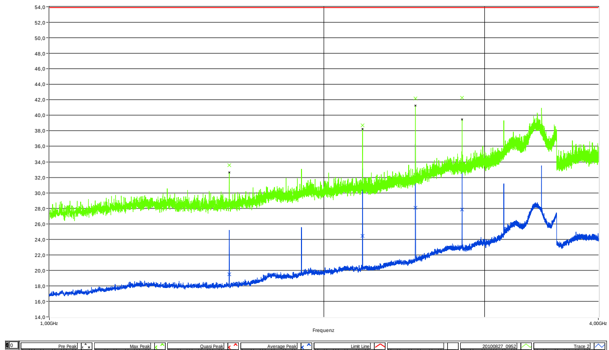
Figure 6-96: Radiated Emissions (1GHz – 4GHz)
