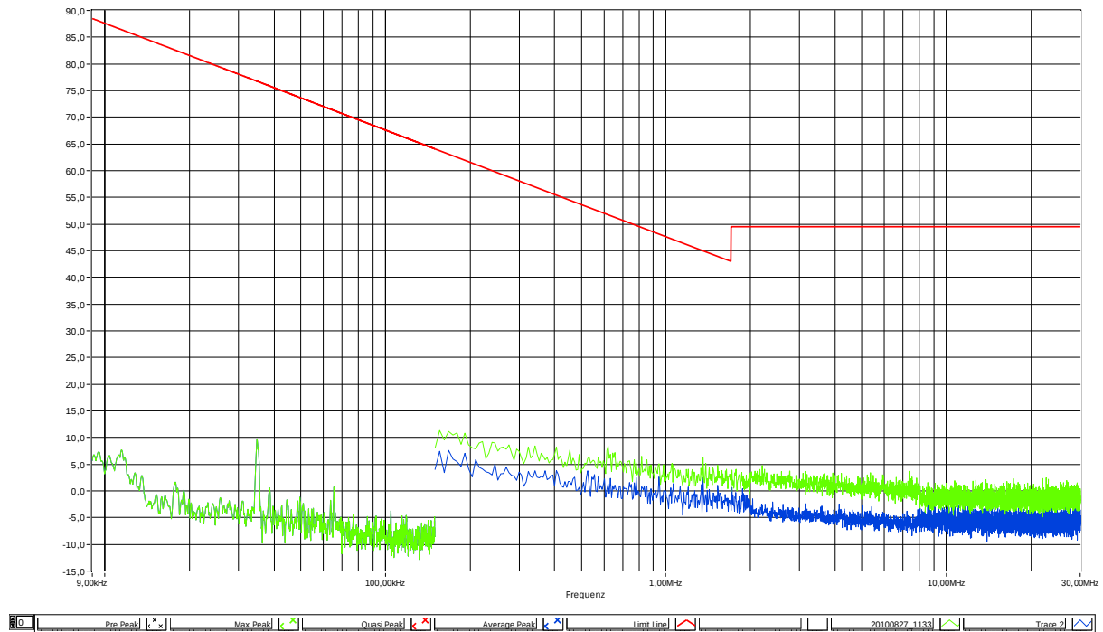
Figure 6-7: Radiated Emissions (9kHz – 30MHz)
