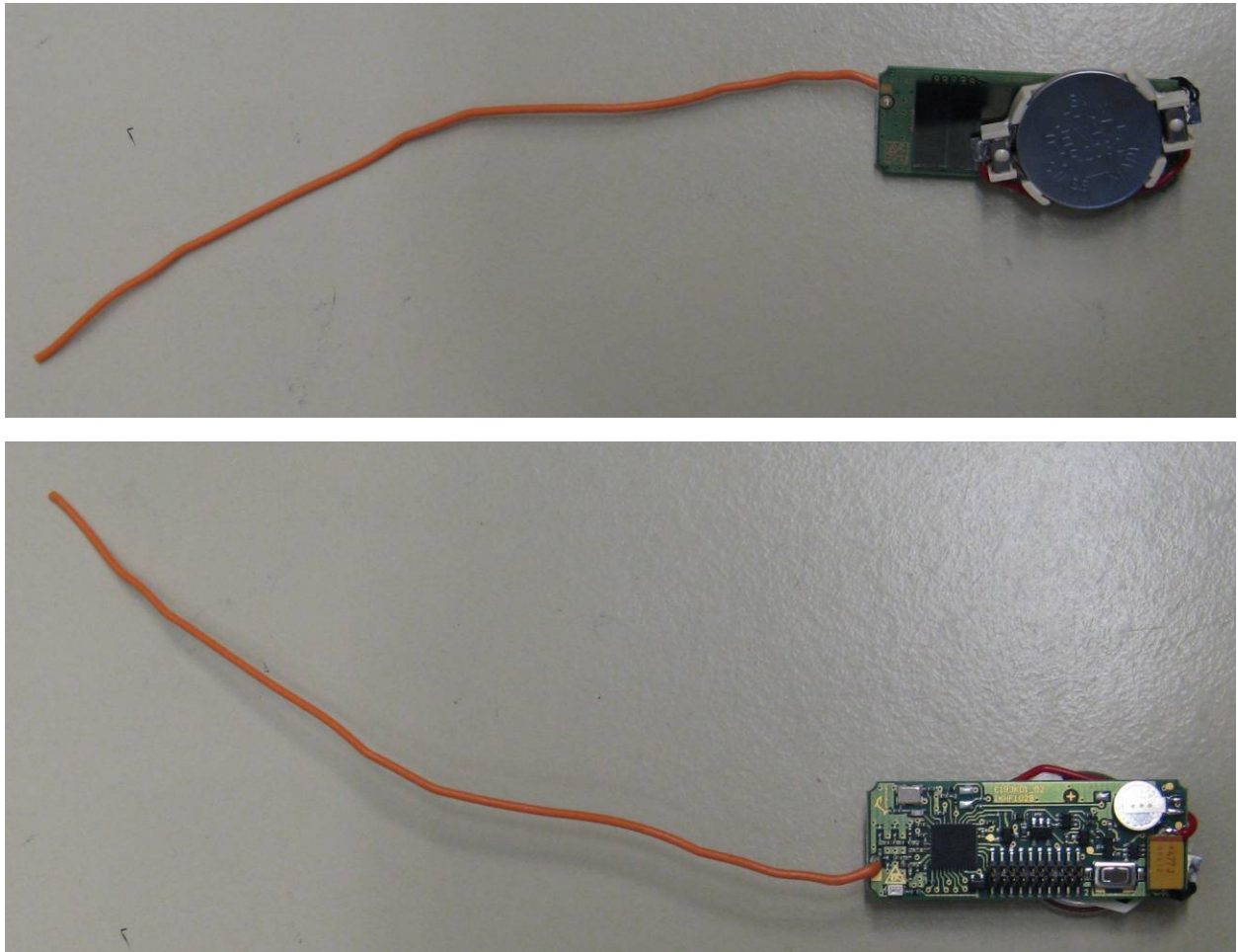
Figure 4-1: Photos of EUT
