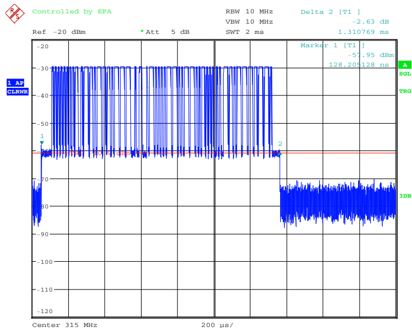
Figure 6-3: Duty Cycle (Complete Pulse train)
