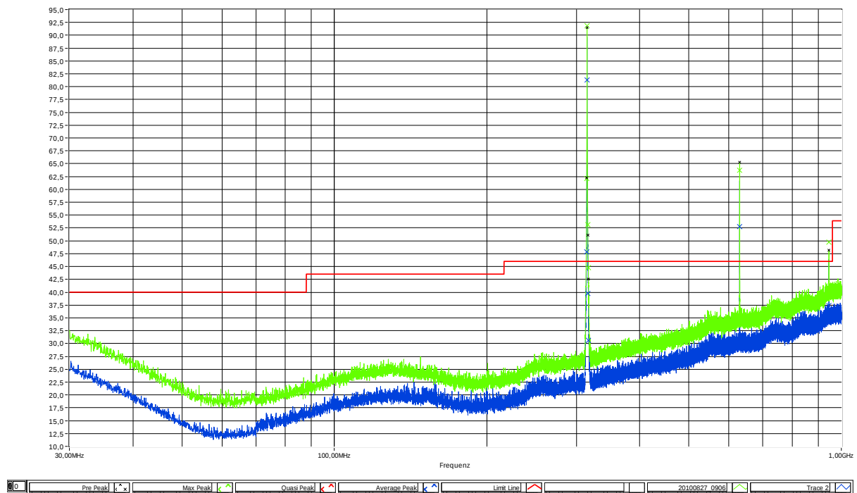
Figure 6-11: Radiated Emissions (30MHz – 1GHz)
