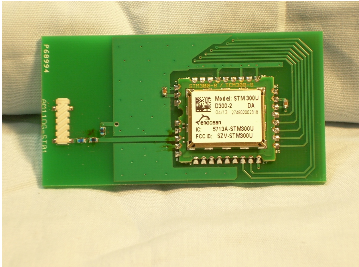
Photograph 4 – Front View of the Module and Antenna
