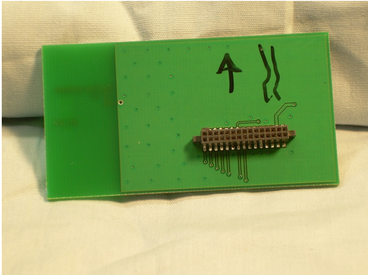
Photograph 5 – Back View of the PCB with Module Interface Connector
