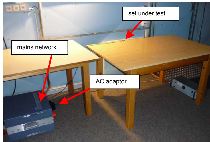
conducted emission 150 kHz - 30 MHz
