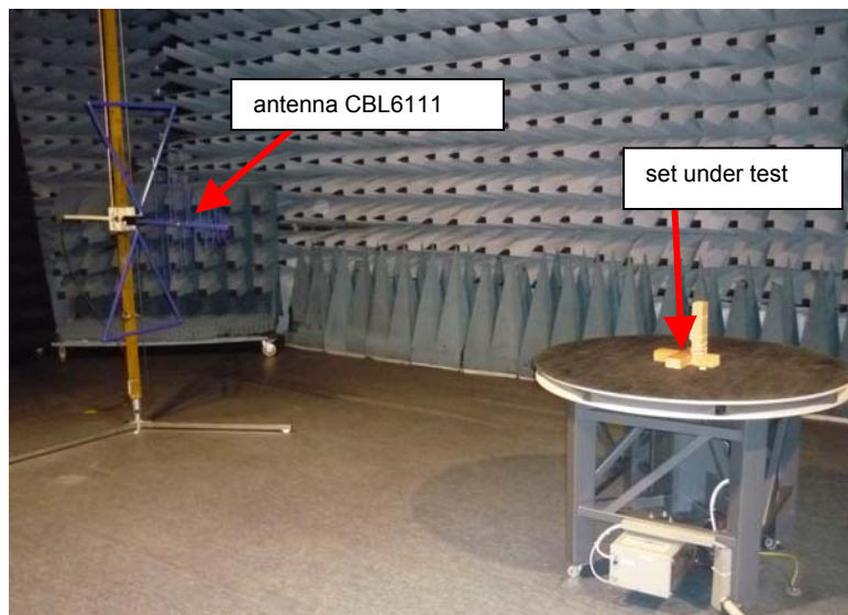
test setup for frequencies between 30MHz and 1000MHz
