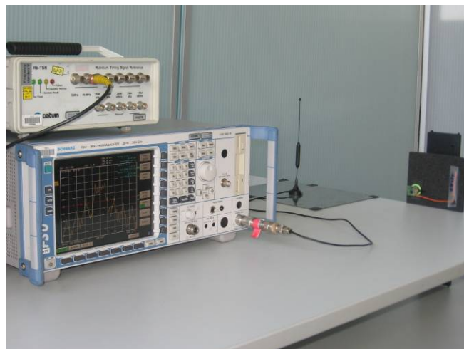
Figure 6-4: Test Configuration – Duty Cycle
