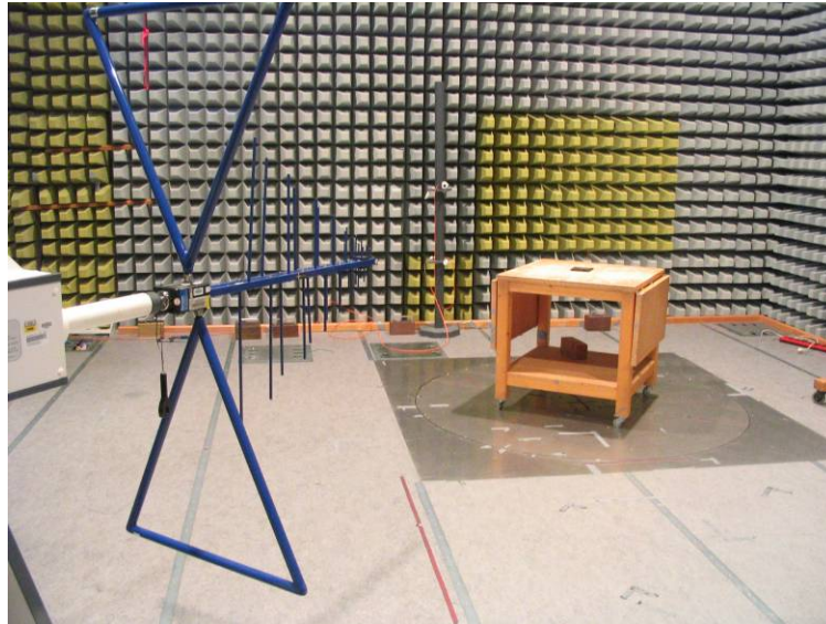
Figure 6-7: Test Configuration – Field Strength of Fundamental Wave
