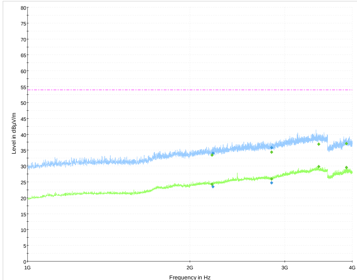
Figure 6-13: Radiated Emissions (1GHz – 4GHz)
