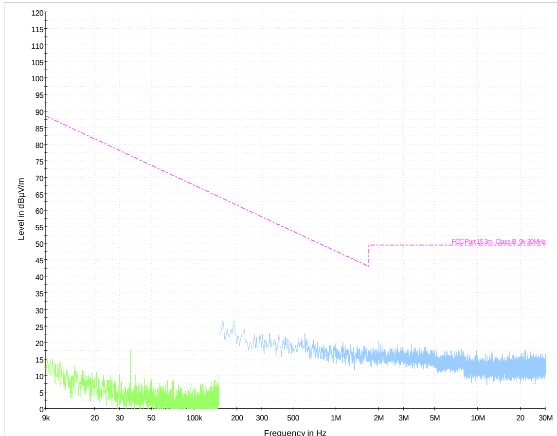
Figure 6-9: Radiated Emissions (9kHz – 30MHz)
