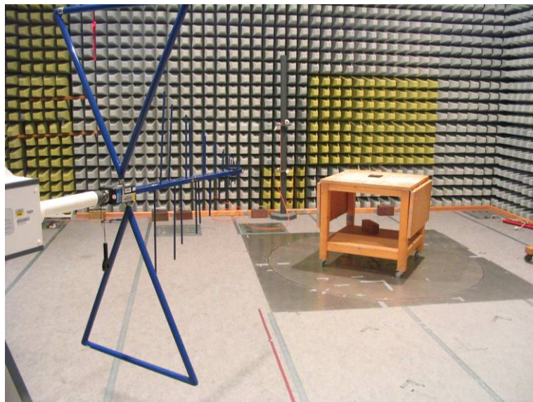
Figure 6-10: Test Configuration – Radiated Emissions (30MHz – 1GHz)
