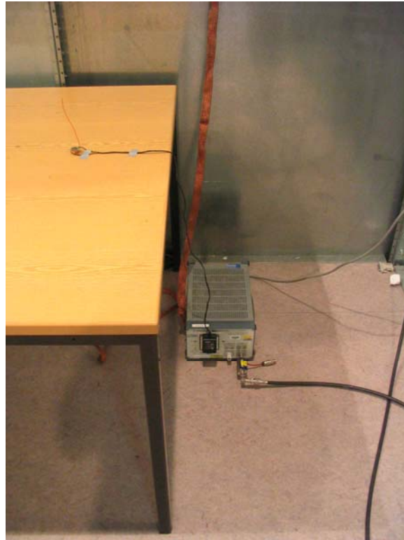
Figure 6-2: Test Configuration – Conducted Emissions (150k – 30MHz)
