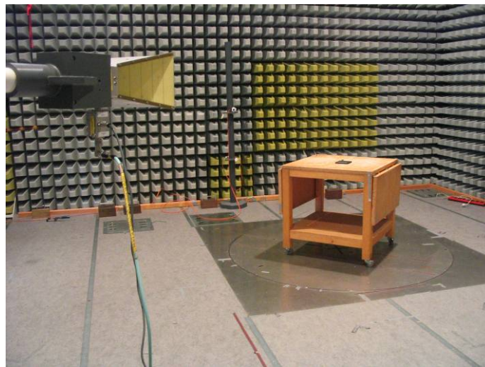
Figure 6-12: Test Configuration – Radiated Emissions (1GHz – 4GHz)
