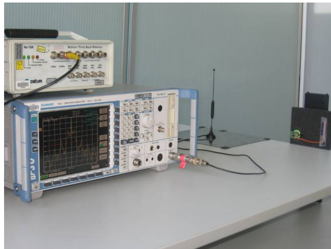
Figure 6-14: Test Configuration – Emission Bandwidth
