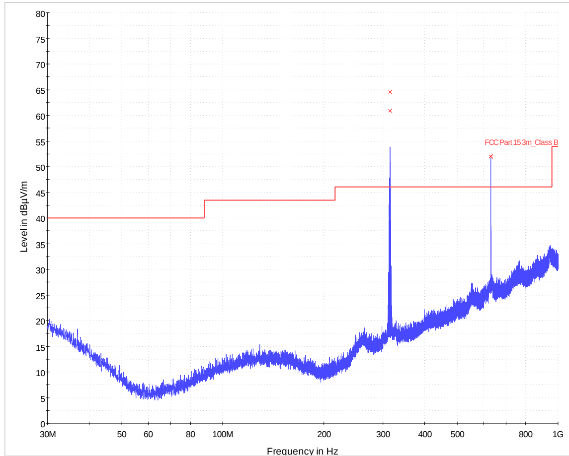
Figure 6-11: Radiated Emissions (30MHz – 1GHz)
