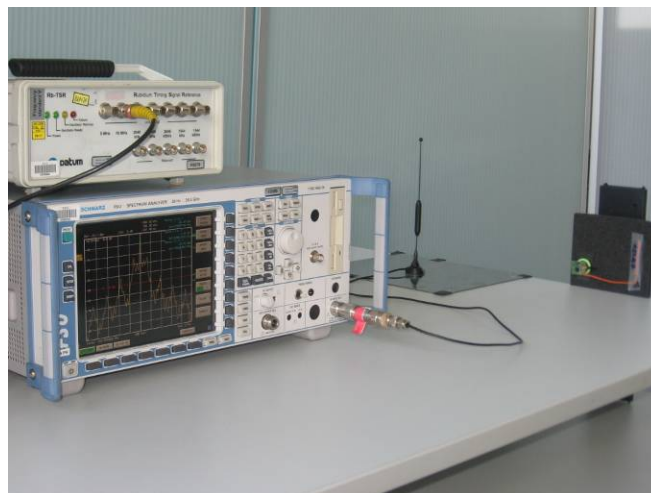
Figure 6-16: Test Configuration – Transmit Duration
