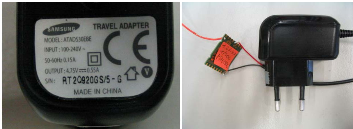
Figure 6-1: Power supply for conducted emission test on AC power port
