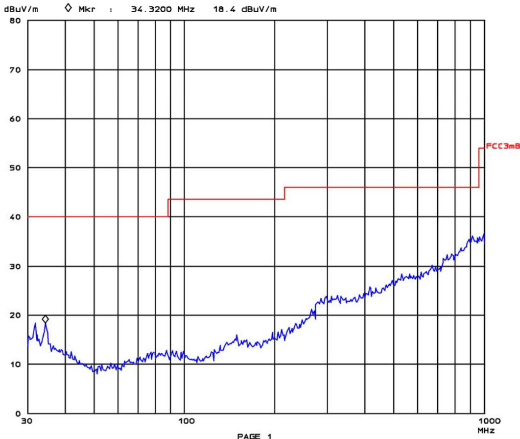
Plot 6.7.3-1: PTM 215Z, Sample #2, pre-scan plot d = 3 m (30 MHz to 1 GHz); channel 11
