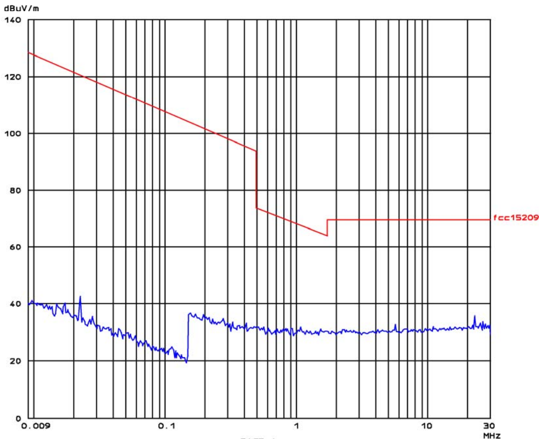
Plot 6.7.2-1: PTM 215Z, Sample #2, Magnetic Field emissions at 3 m distance; channel 11
