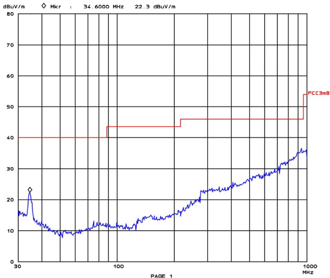
Plot 6.7.3-2: PTM 215Z, Sample #2, pre-scan plot d = 3 m (30 MHz to 1 GHz); channel 20
