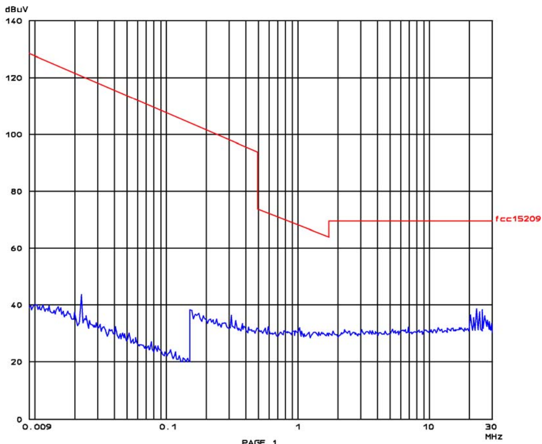
Plot 6.7.2-3: PTM 215Z, Sample #2, Magnetic Field emissions at 3 m distance; channel 25
