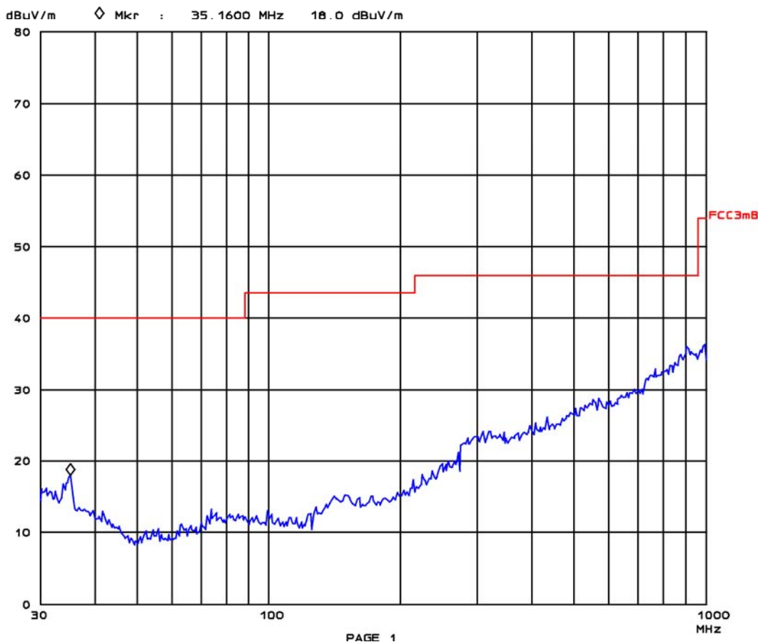
Plot 6.7.3-3: PTM 215Z, Sample #2, pre-scan plot d = 3 m (30 MHz to 1 GHz); channel 25
