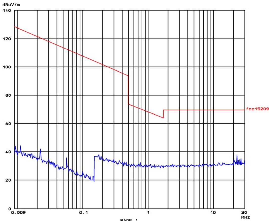
Plot 6.7.2-2: PTM 215Z, Sample #2, Magnetic Field emissions at 3 m distance; channel 20
