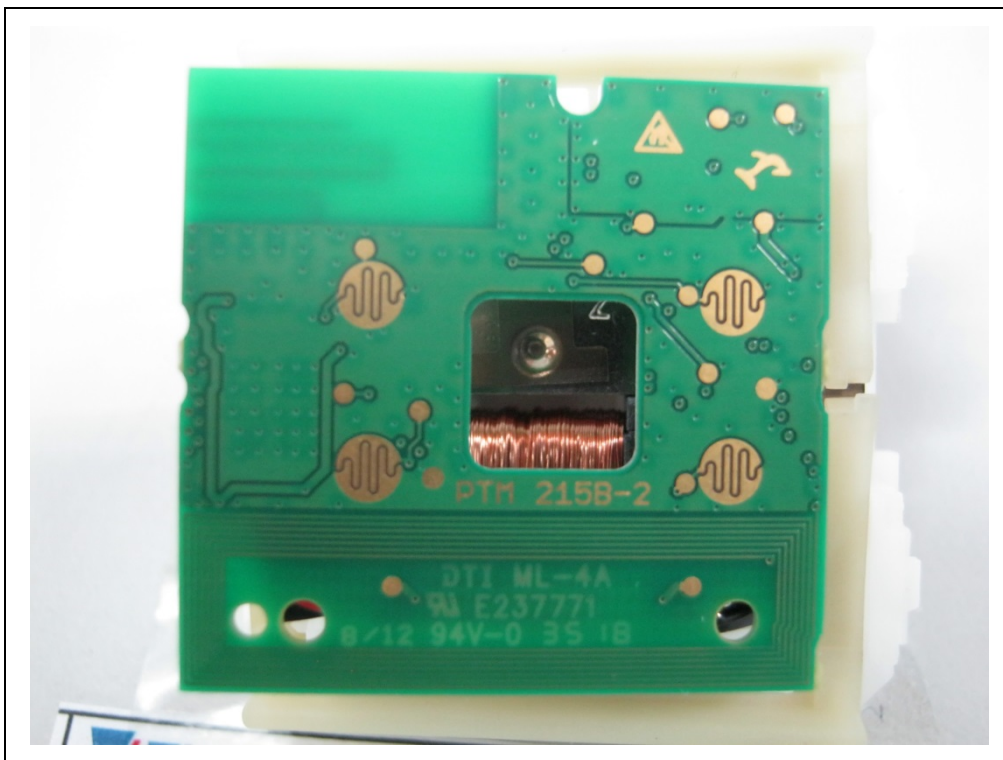
Photograph A3-2: EUT#1, detail on PCB top
