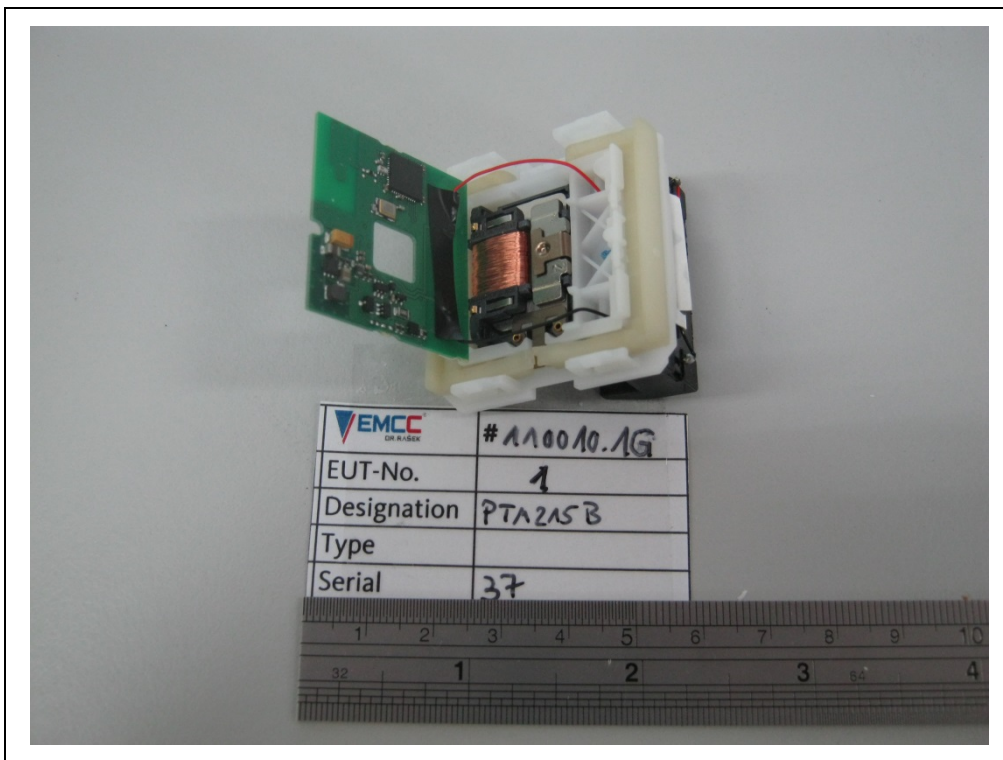
Photograph A3-4: EUT#1, PCB removed view on "external" power generator
