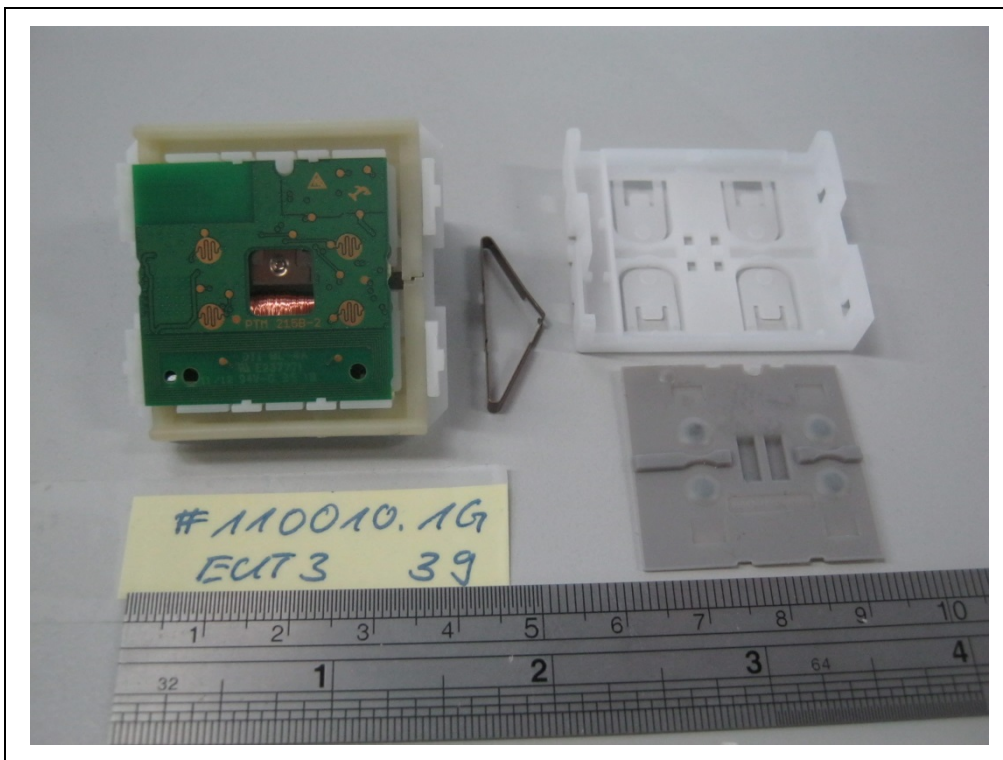
Photograph A3-6: EUT#3, with cover removed
