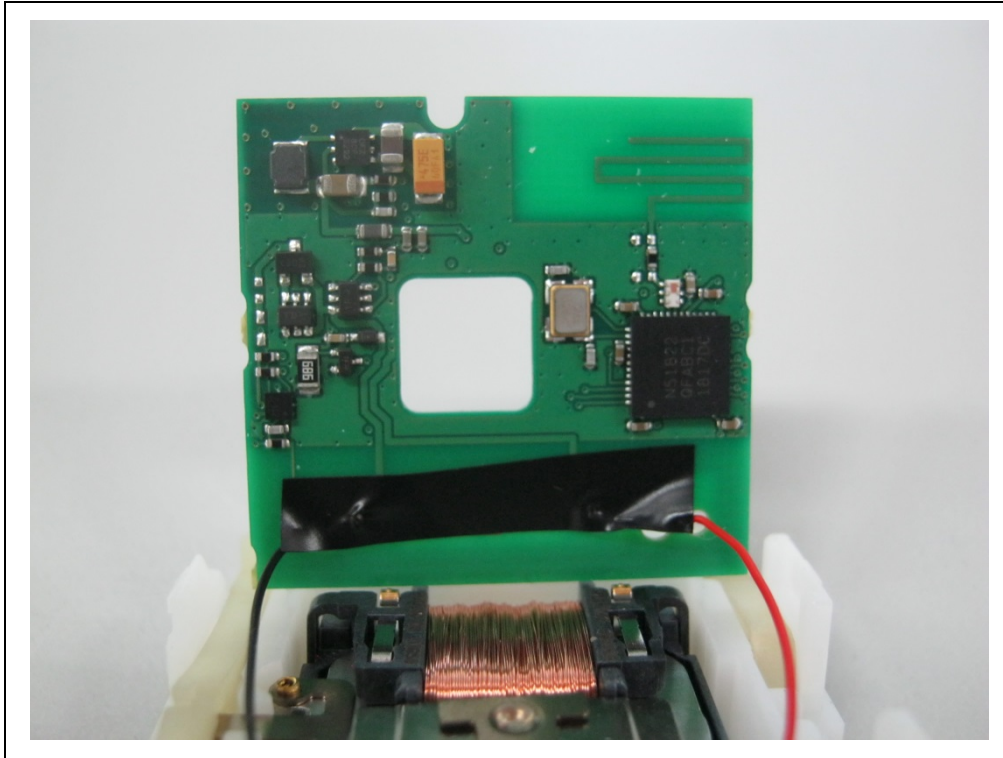
Photograph A3-3: EUT#1, detail on PCB bottom
