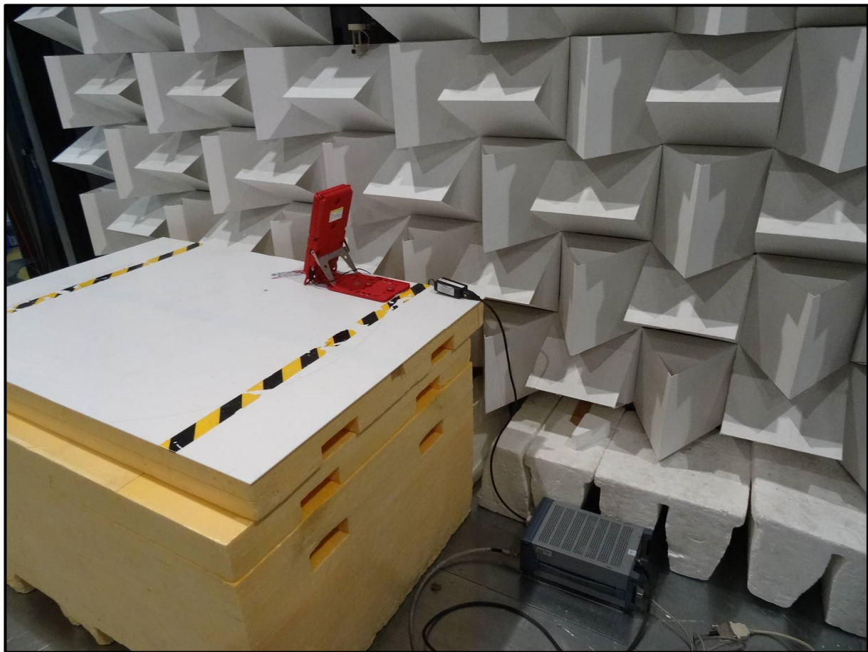
AC Conducted Spurious Emission
