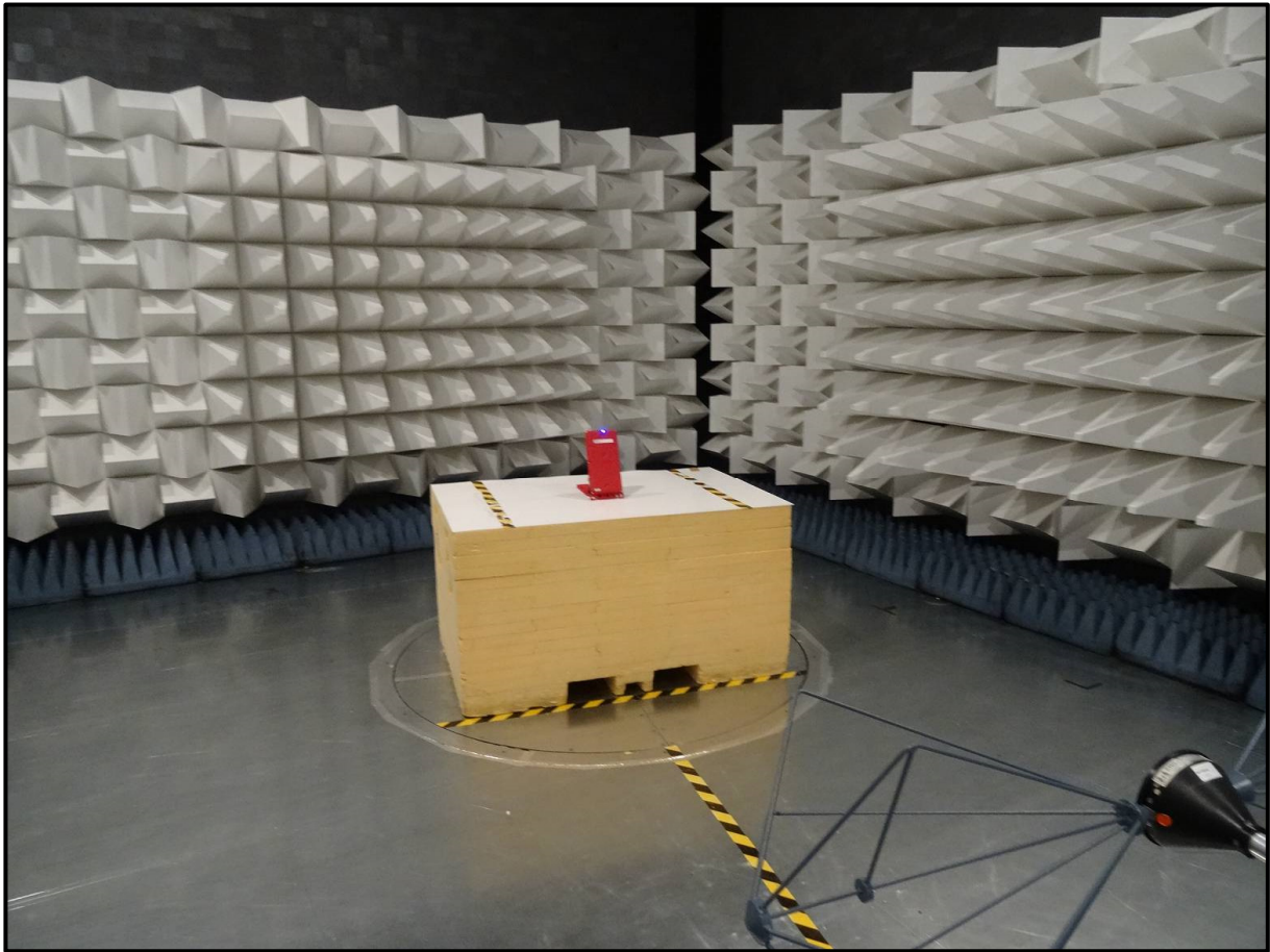
Radiated Spurious Emission from 30 MHz to 200 MHz
