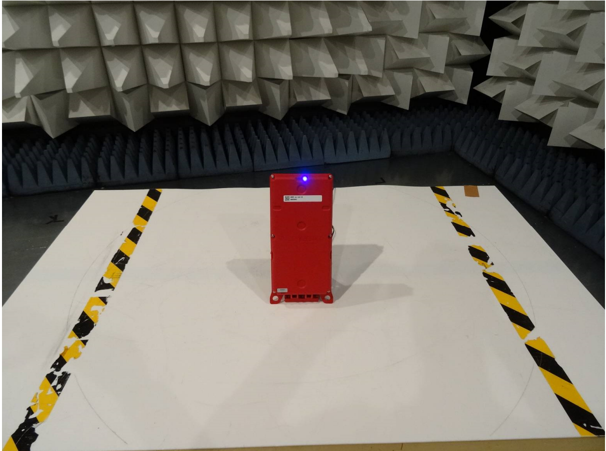
Radiated Spurious Emissions from 30MHz to 1GHz
