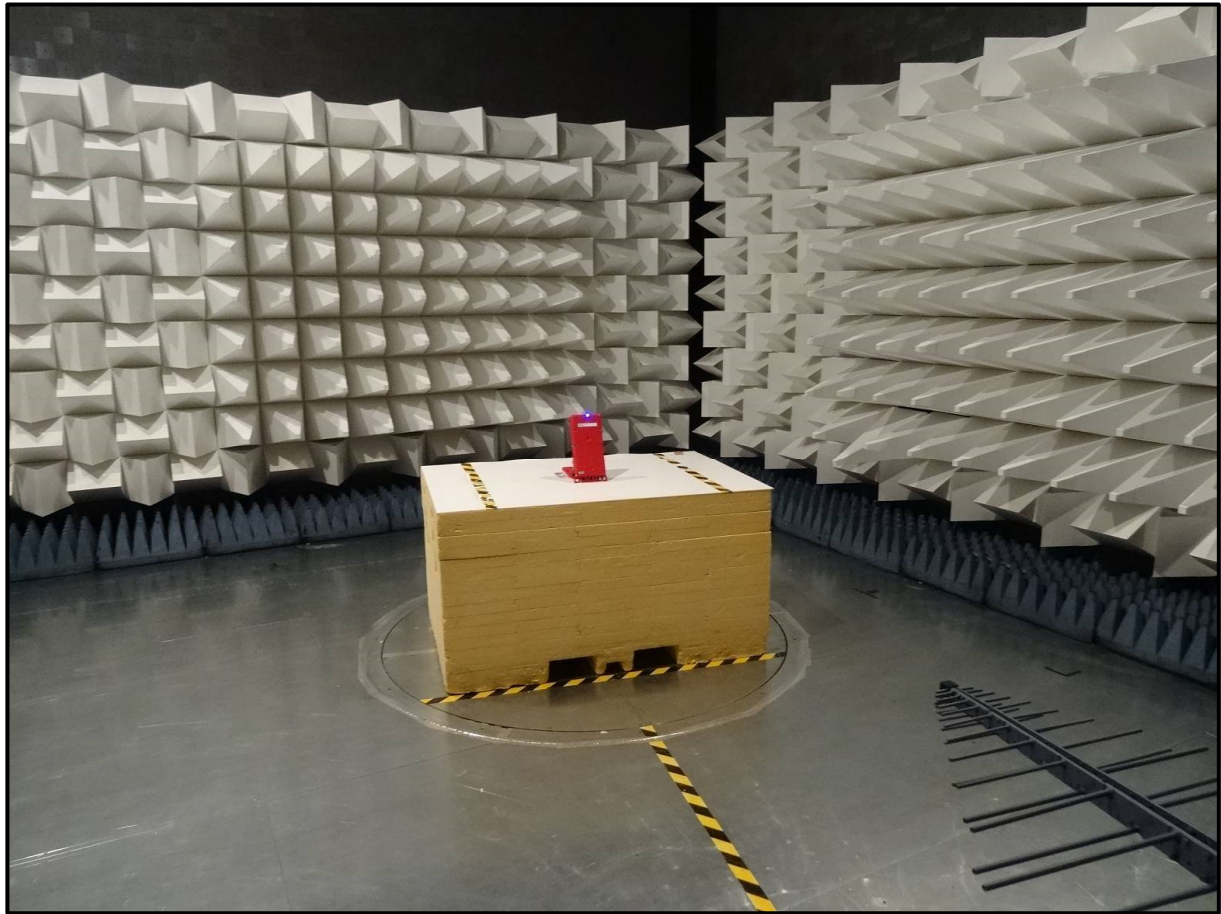
Radiated Spurious Emission from 200 MHz to 1000 MHz
