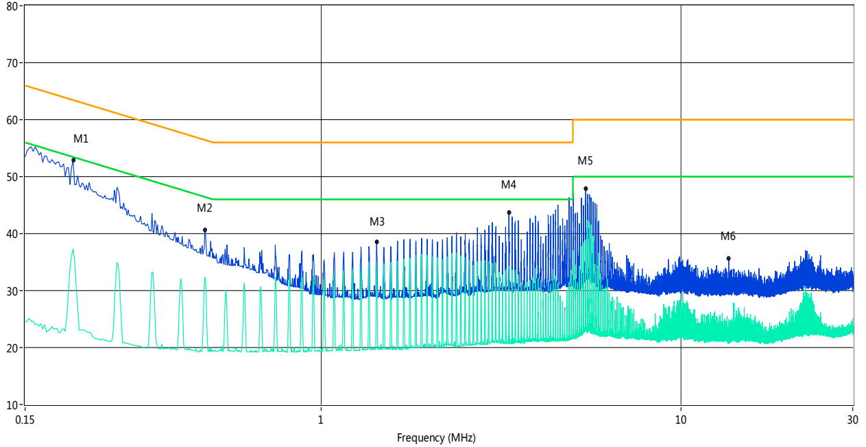
802.11b HIGH CHANNEL PHASE L
