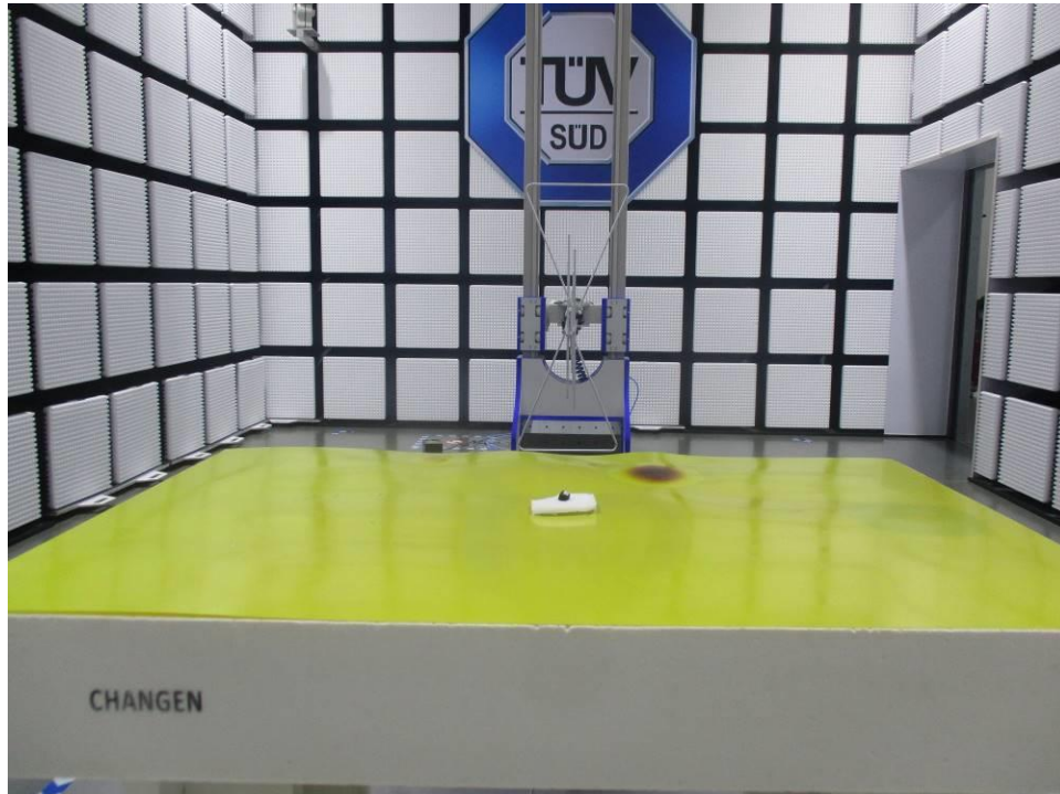
Radio Emission (30MHz-1GHz)
