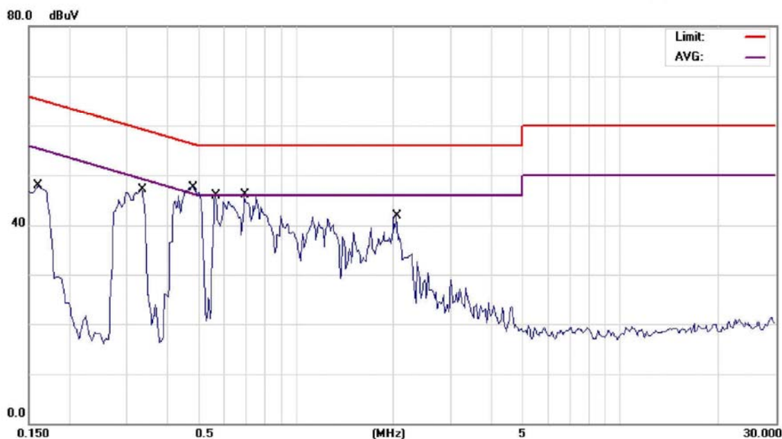
Conducted Emission Measurement
