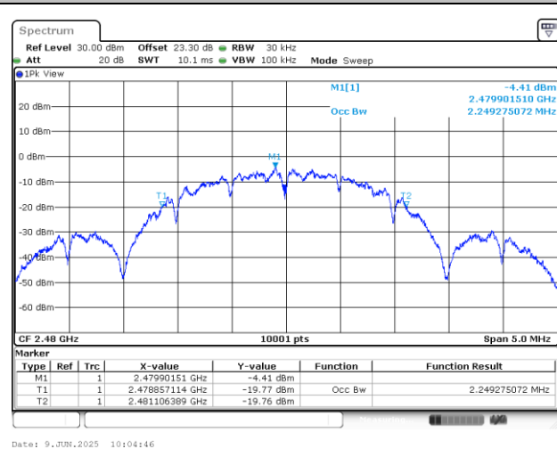
99% Occupied Bandwidth Plot on Channel 26
