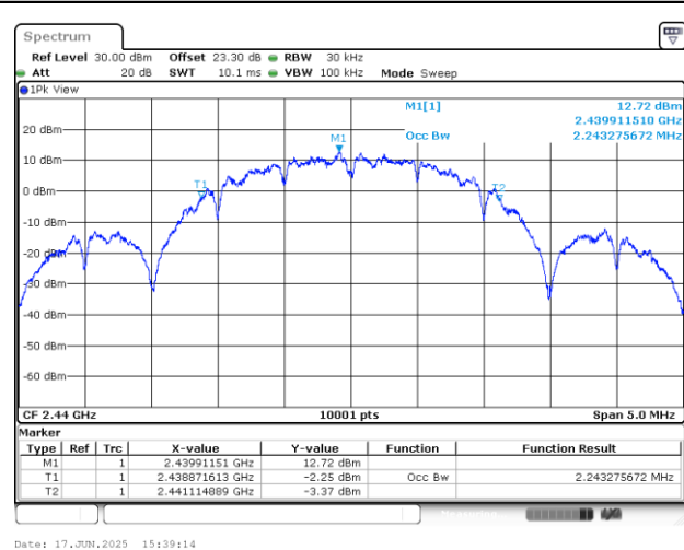
99% Occupied Bandwidth Plot on Channel 18
