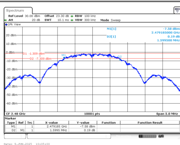
6 dB Bandwidth Plot on Channel 26
