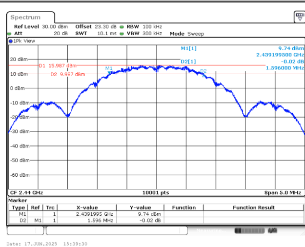
6 dB Bandwidth Plot on Channel 18
