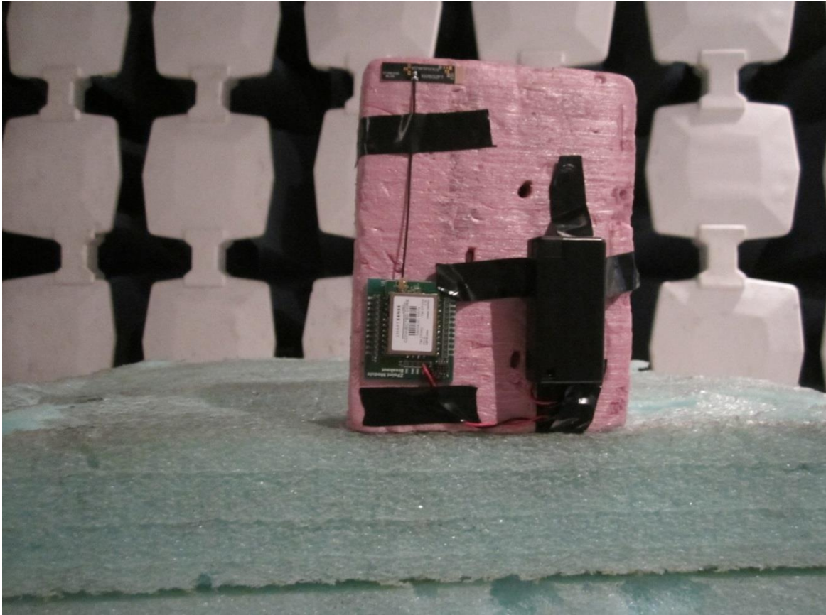
X-orientation (resulted in highest emissions)
