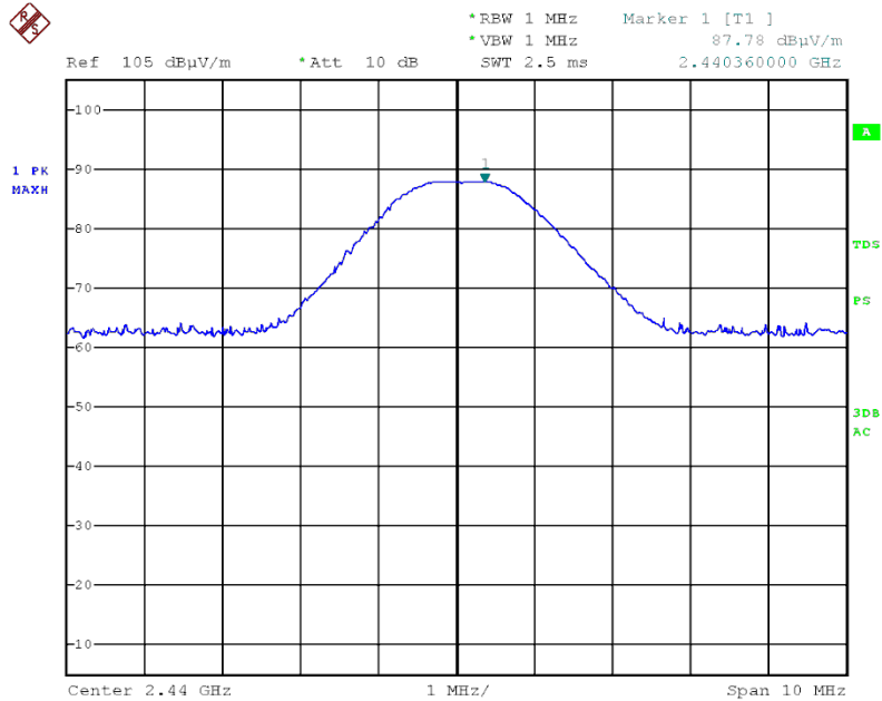
Figure 15 2440.0 MHz – Vertical
