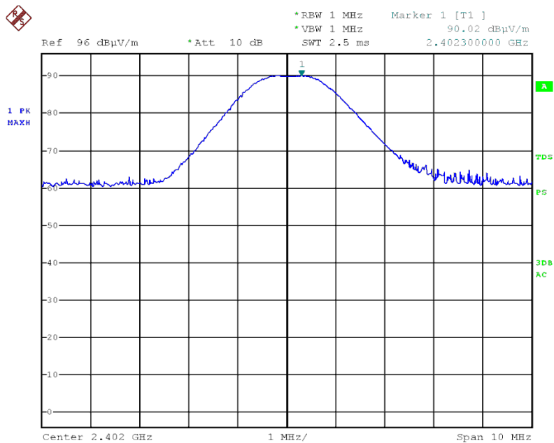
Figure 13 2402.0 MHz – Vertical
