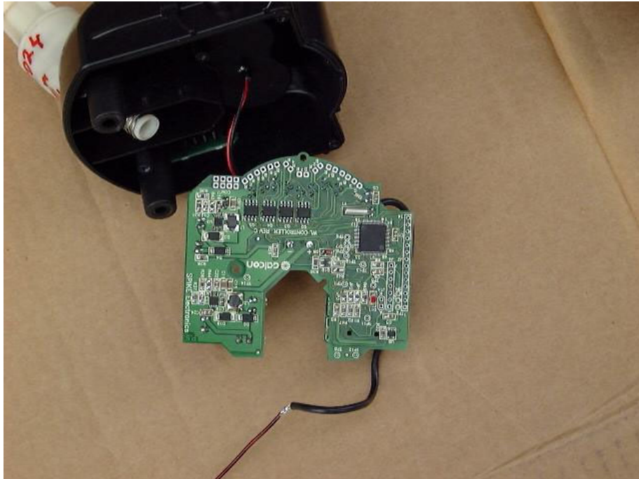
Figure 3 PCB 1 Side 2
