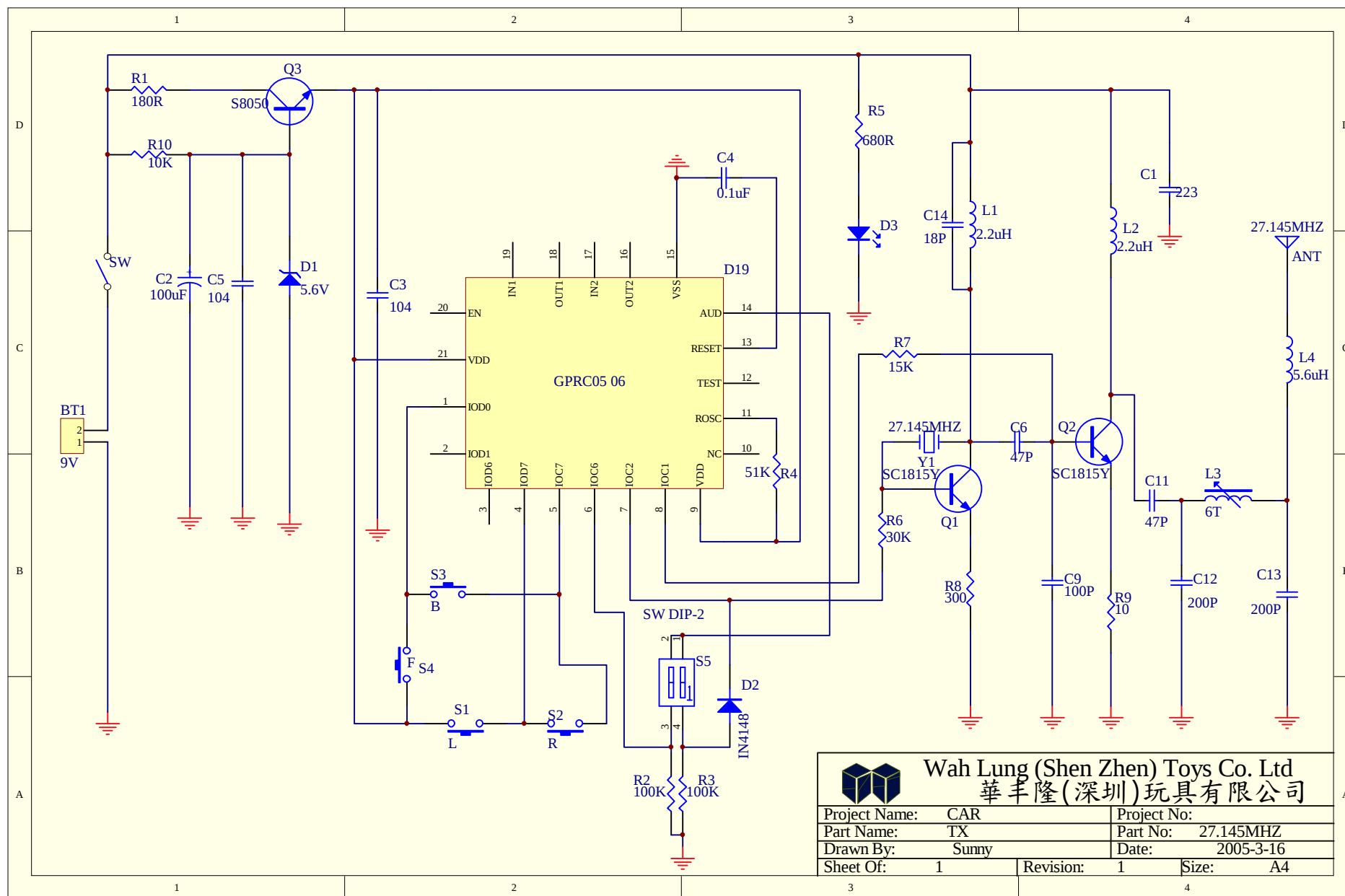
27.145MHZ TX CIRCUIT SCHEMATIC
