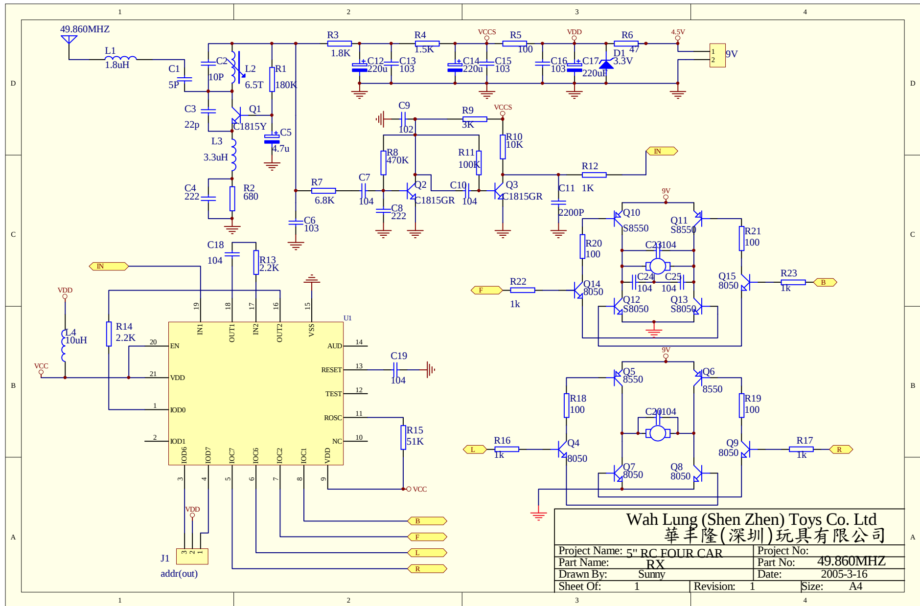
49.860MHZ RX CIRCUIT SCHEMATIC
