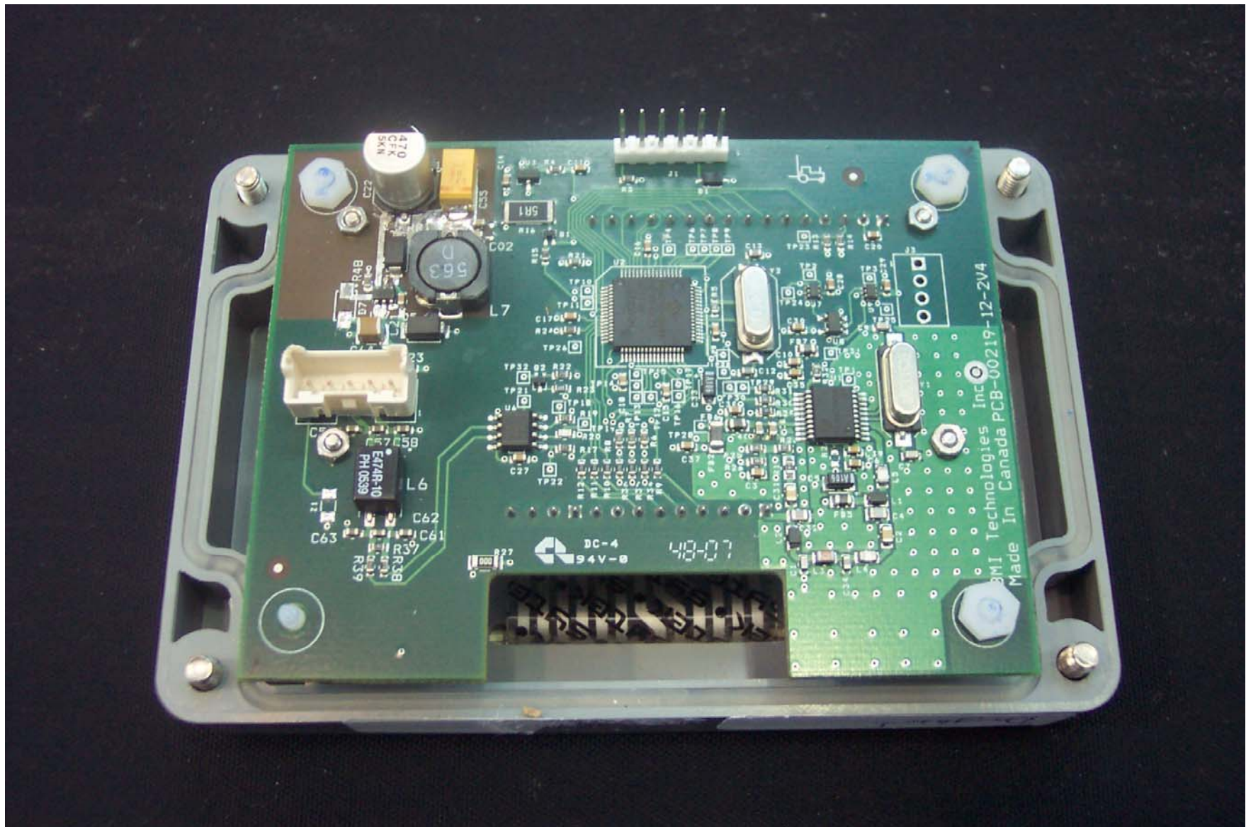
Figure 1: Component Side, main board
