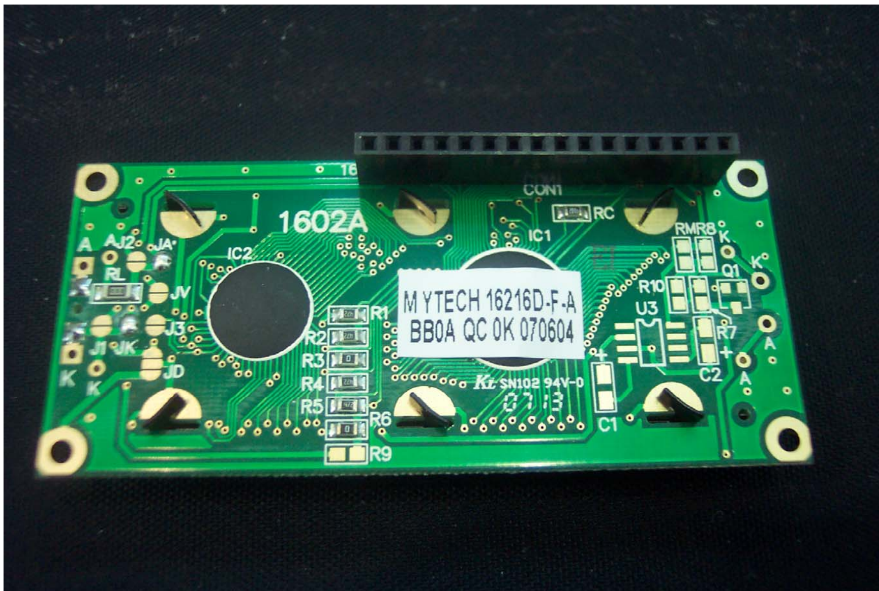
Figure 3: Component Side, daughter board
