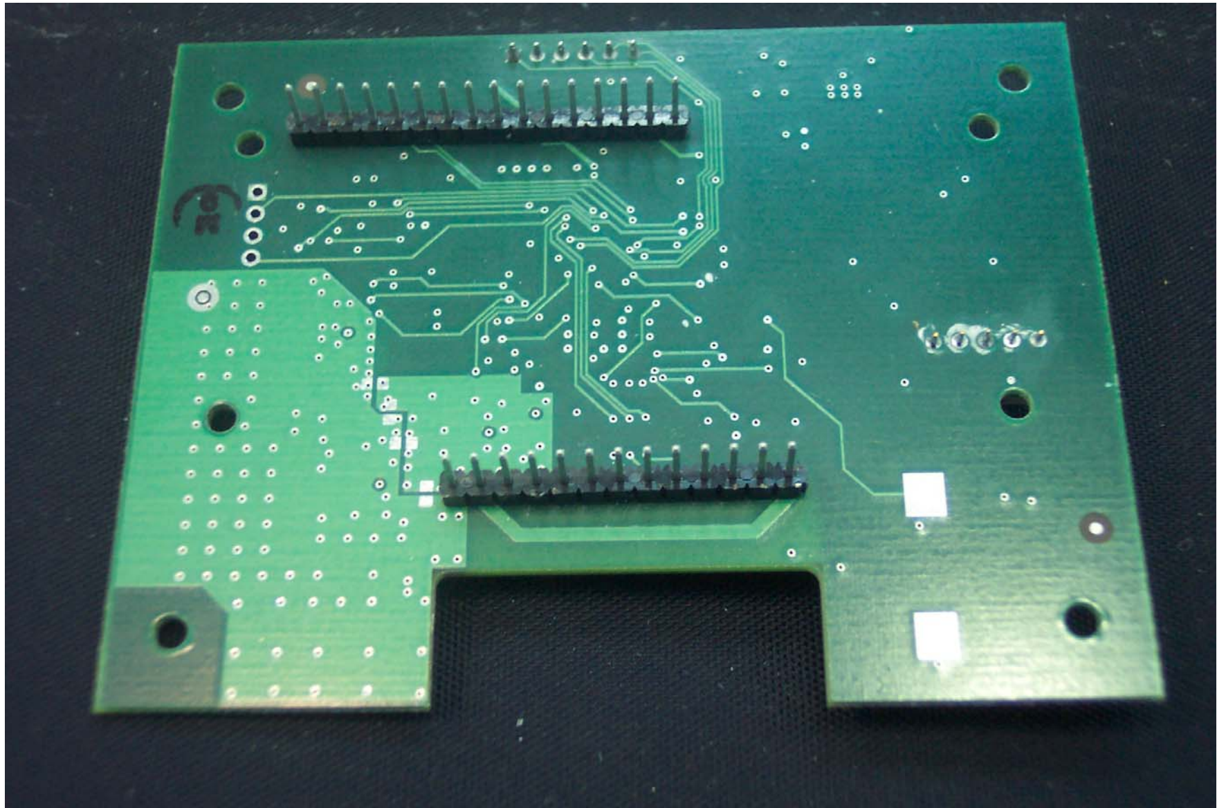
Figure 4: Solder side, main board
