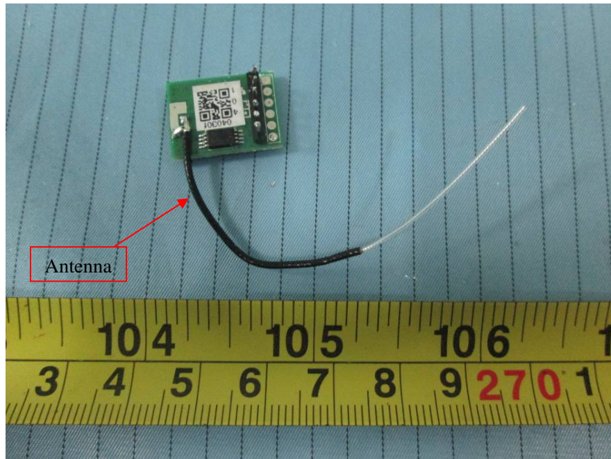
EUT – BT Main Board View
