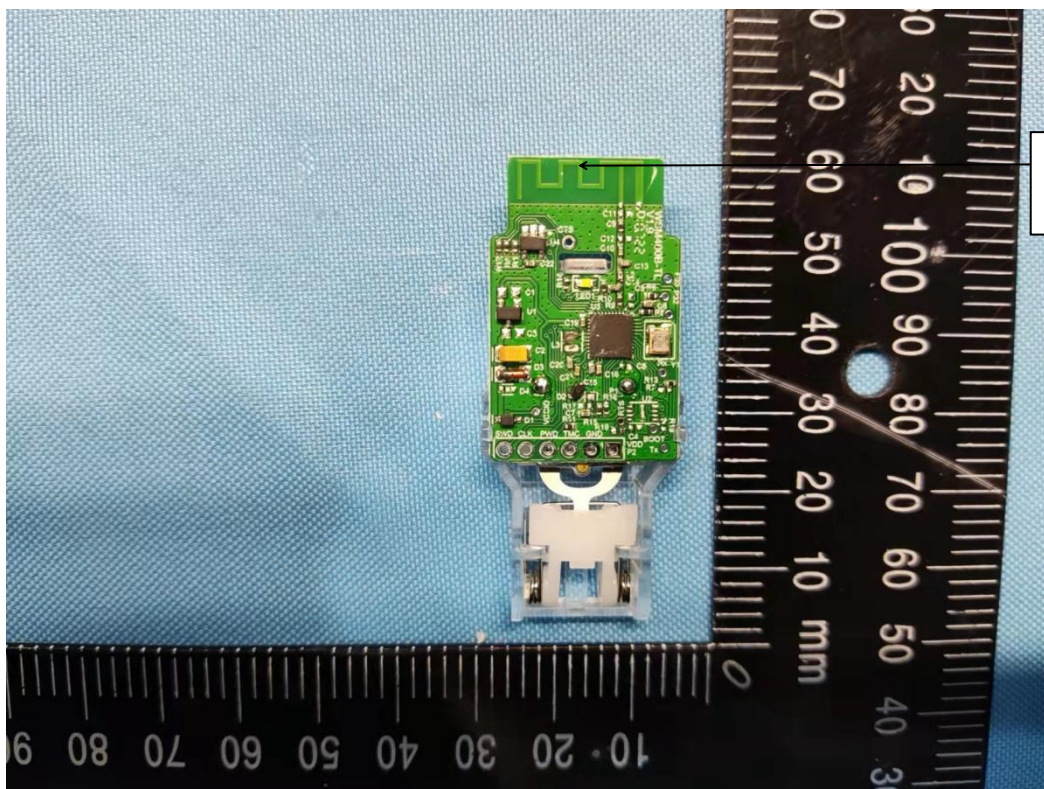
BT Antenna
