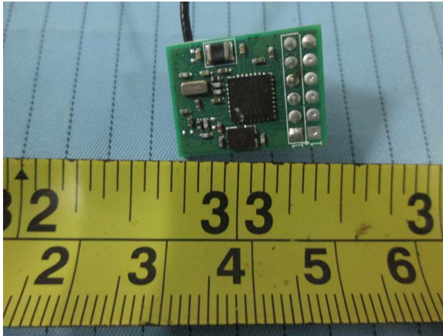
EUT – BT Main Board Top View
