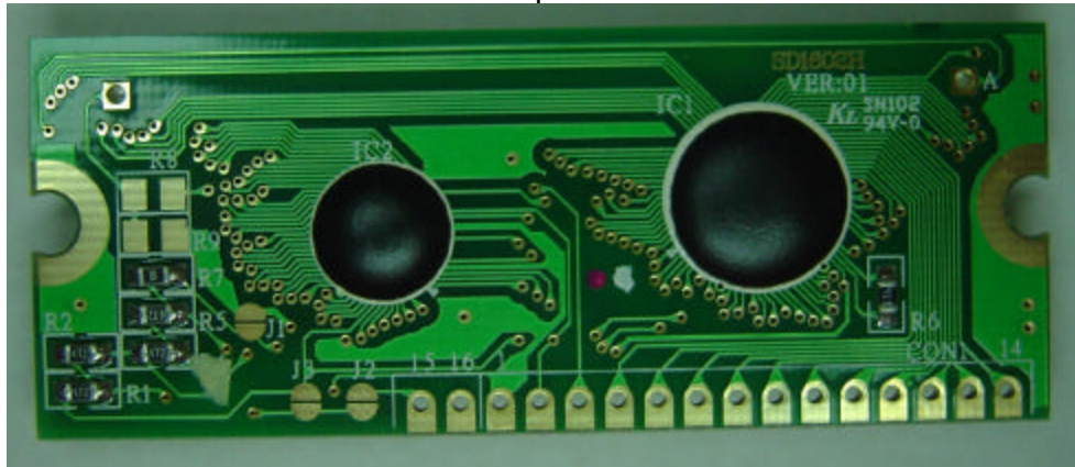
LCD-Component Side
