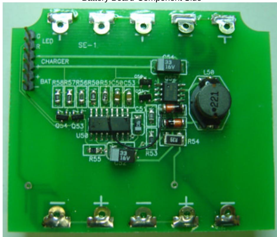
Battery Board-Component Side
