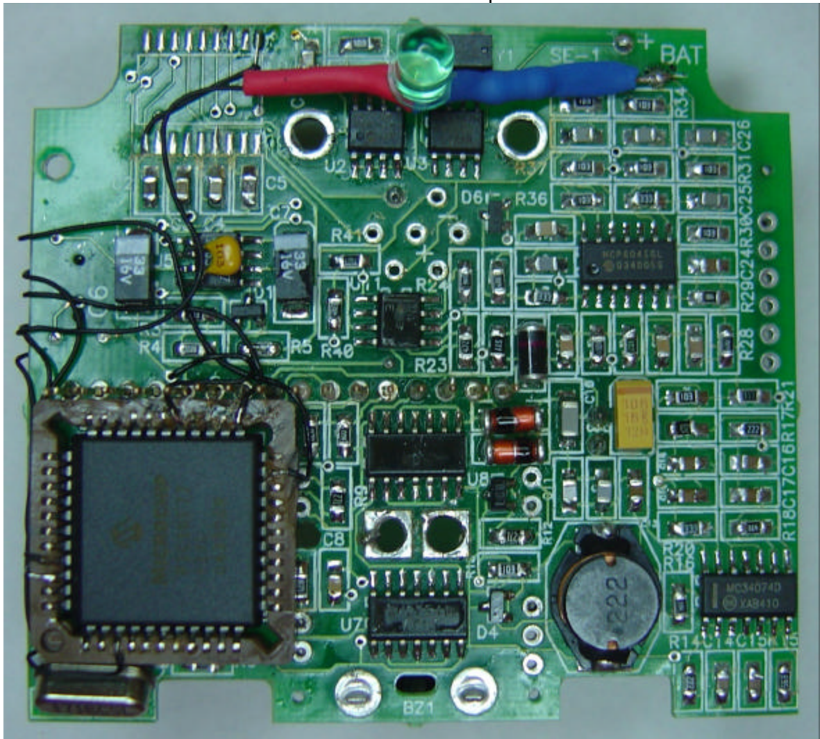
Main board with Reader-Component Side
