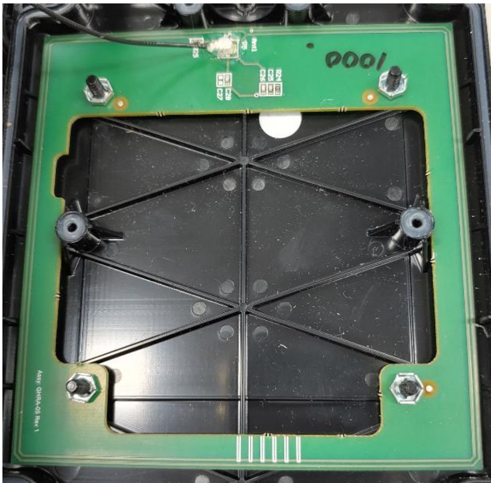
13.56 MHz Antenna
