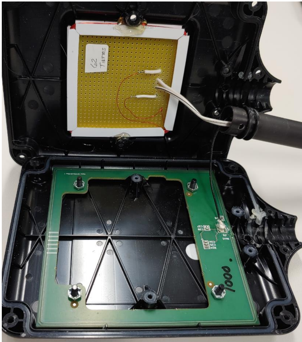
Antennas installed
