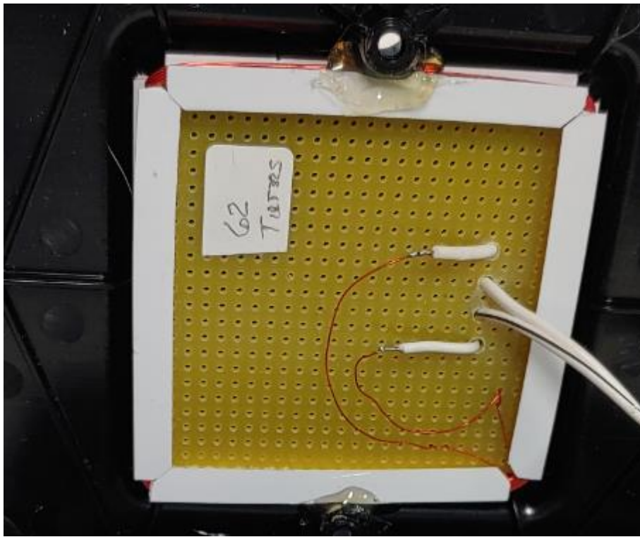
134 kHz Antenna
