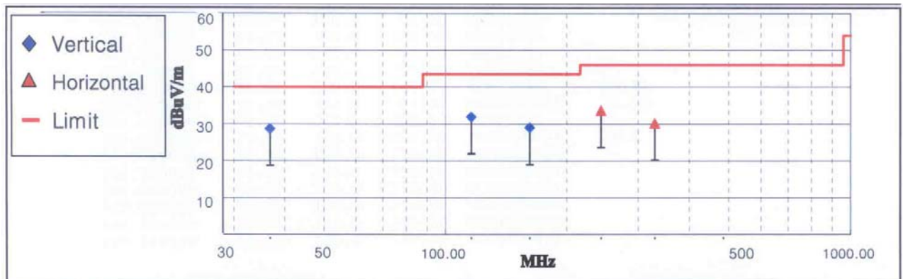
< Fig 8. Radiated emission result _ External input mode (DVD play) >
