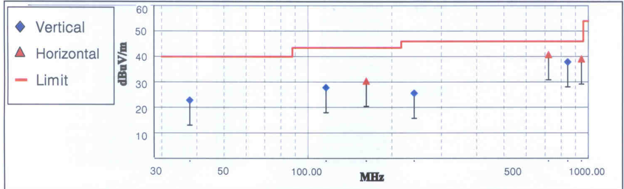
< Fig 4. Radiated emission result _ Download mode >
