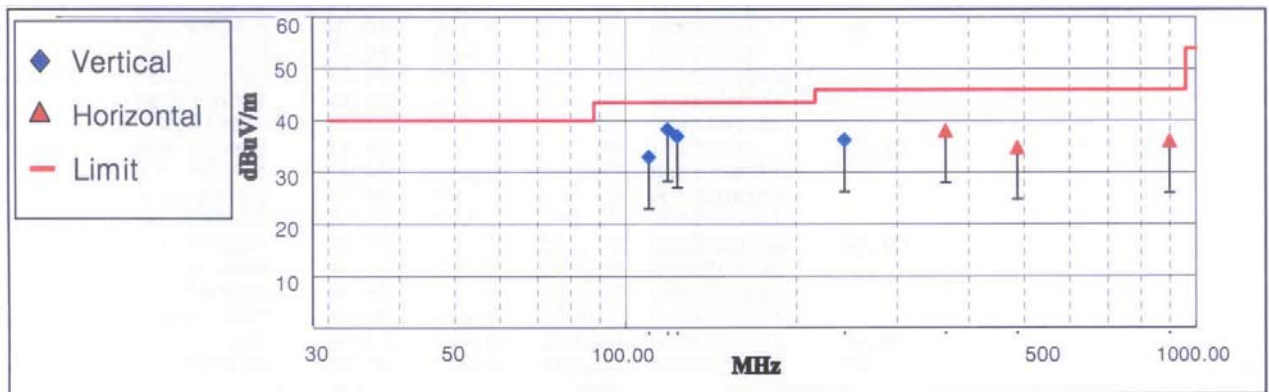
< Fig 6. Radiated emission result _ Video file play mode >
