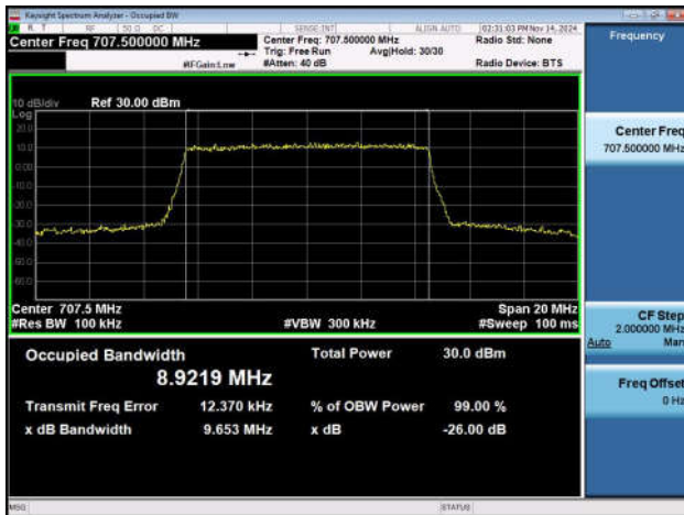
Band12-10MHz-QPSK-23095-50RB#0-PASS
