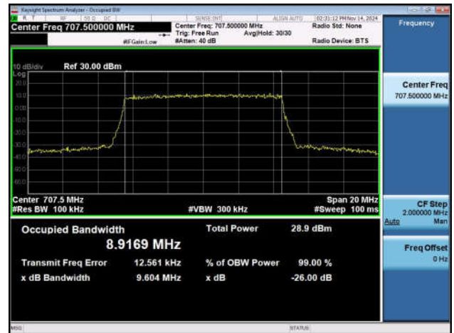
Band12-10MHz-16QAM-23095-50RB#0-PASS
