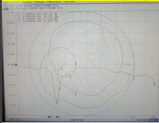
WIFI ANT (size)
