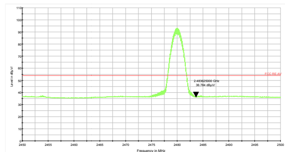
DH5-Channel 78: Average
