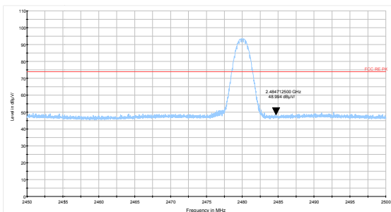
DH5-Channel 78: Peak
