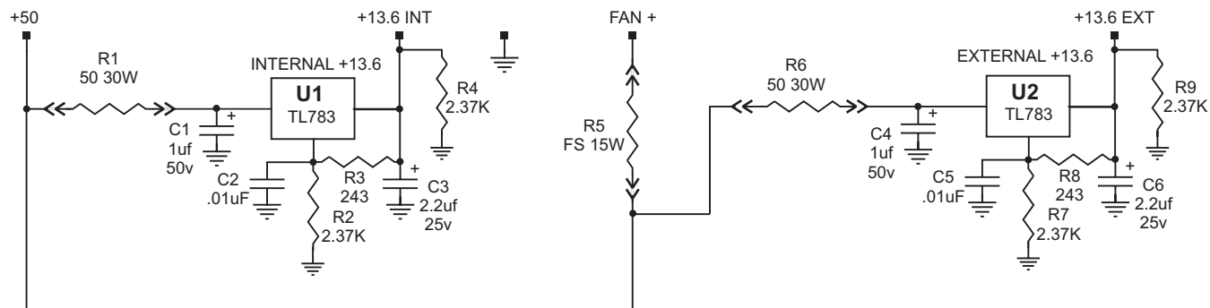
INTERNAL & EXTERNAL 13.6v REGULATORS AND FAN DROPPING RESISTOR
