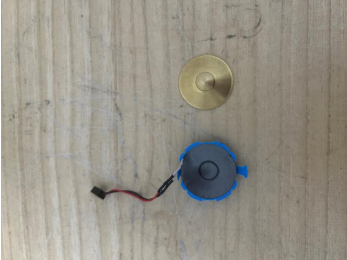
Internal View of EUT-13
