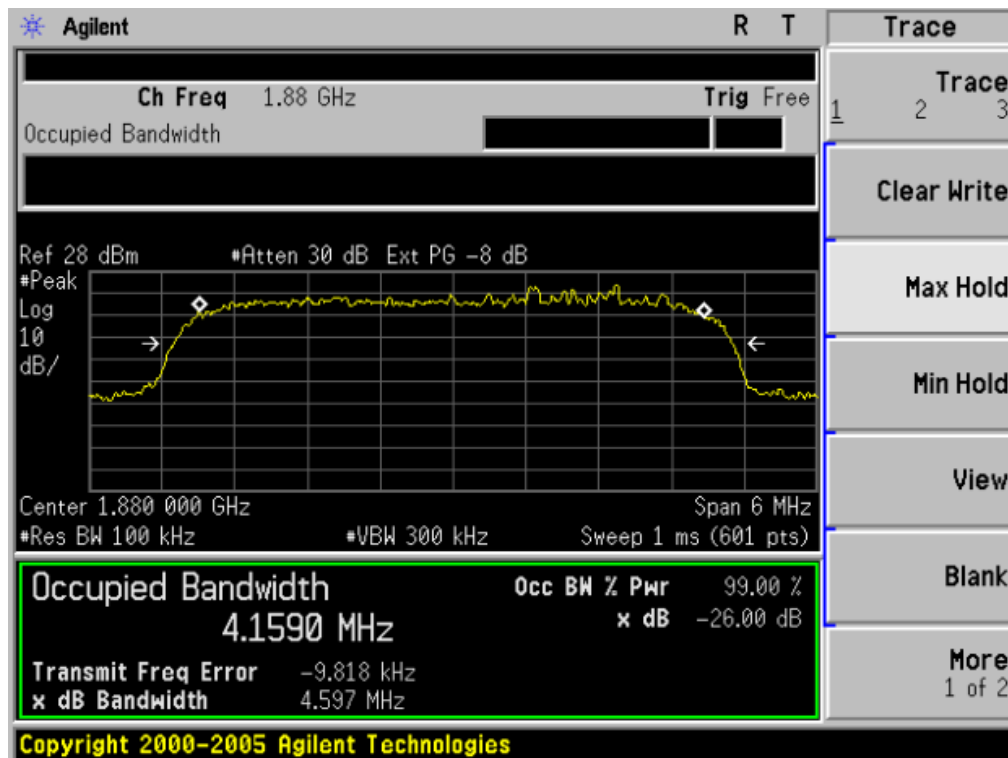
Occupied Bandwidth (99%) UMTS band II CH 9400
