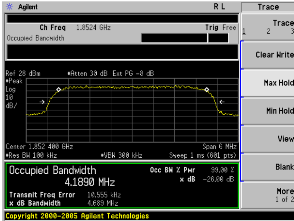
Occupied Bandwidth (99%) UMTS band II CH 9262
