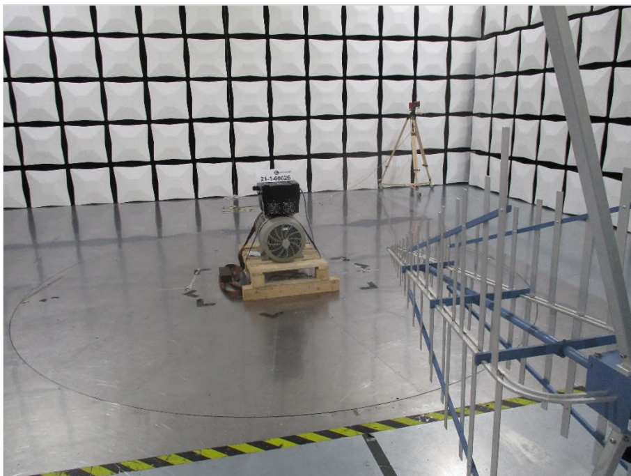
Photograph 2: Radiated emission measurements test set-up Rear side view
