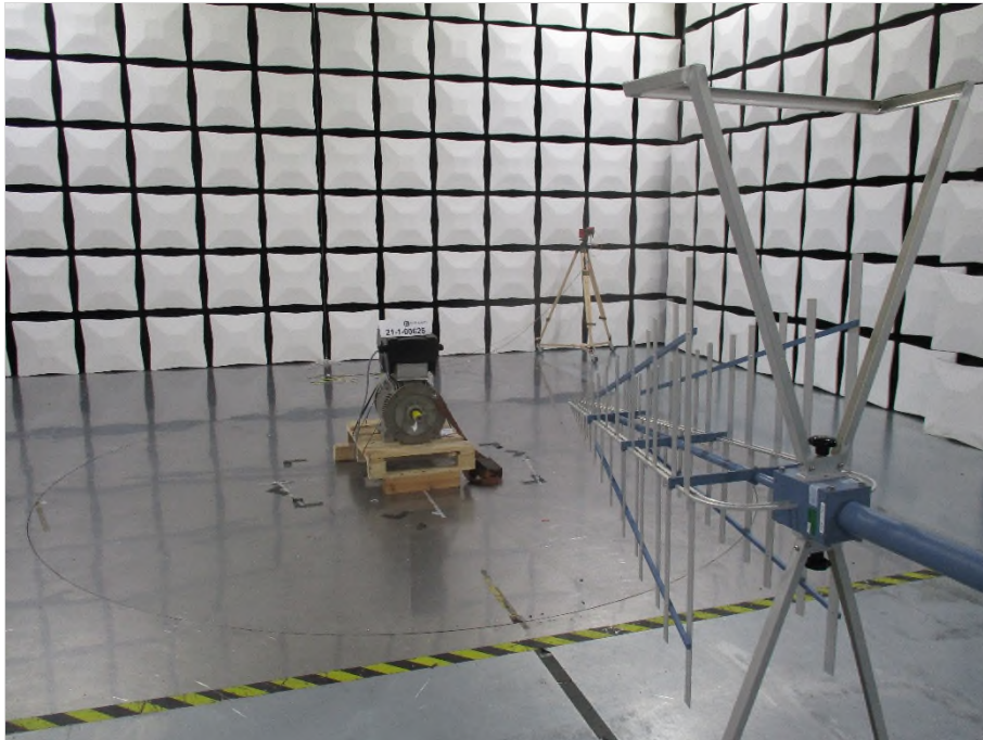
Photograph 3: Radiated emission measurements test set-up Front side view
