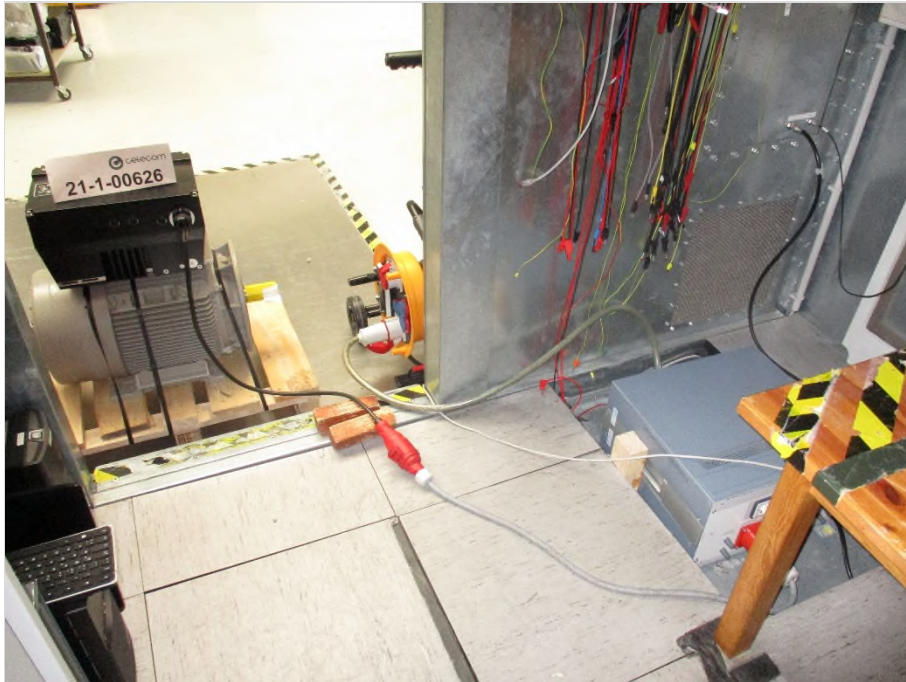
Photograph 1: Mains conducted emission measurements test set-up
