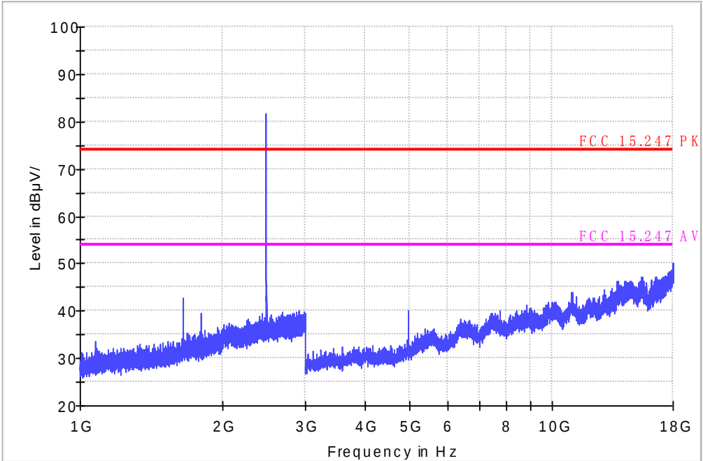
FCC Electric Field Strength 1-18GHz operate on 2.4GHz
