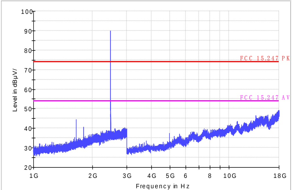
FCC Electric Field Strength 1-18GHz operate on 2.4GHz
