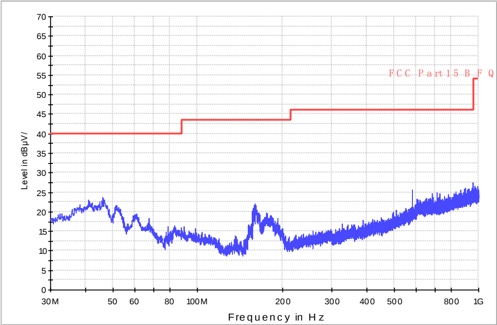
Field strength 30M-1GHz 1F 3m chamber
