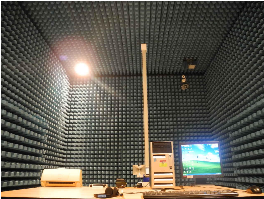
Radiated Emission above 1GHz Front
