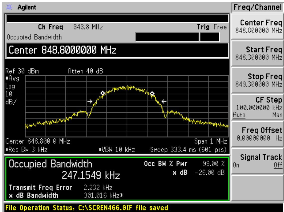
GSM 850+EGPRS CH251 Occupied Bandwidth
