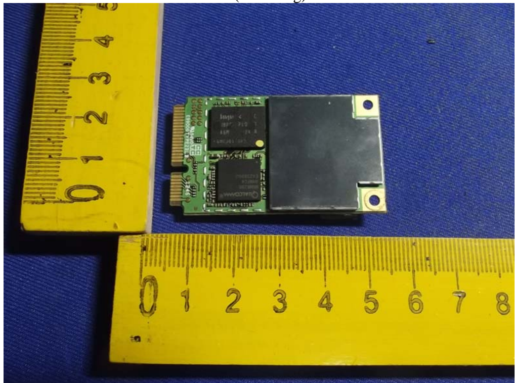
Figure 14 PCB of the 3G Module-Front View (Shielding)
