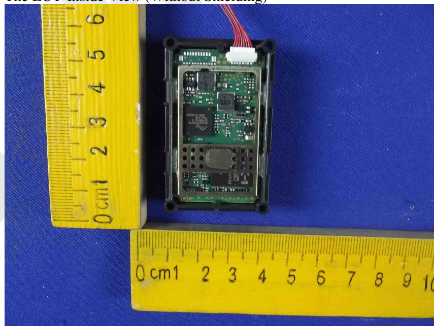
Figure 10 The EUT-Inside View (Without Shielding)
