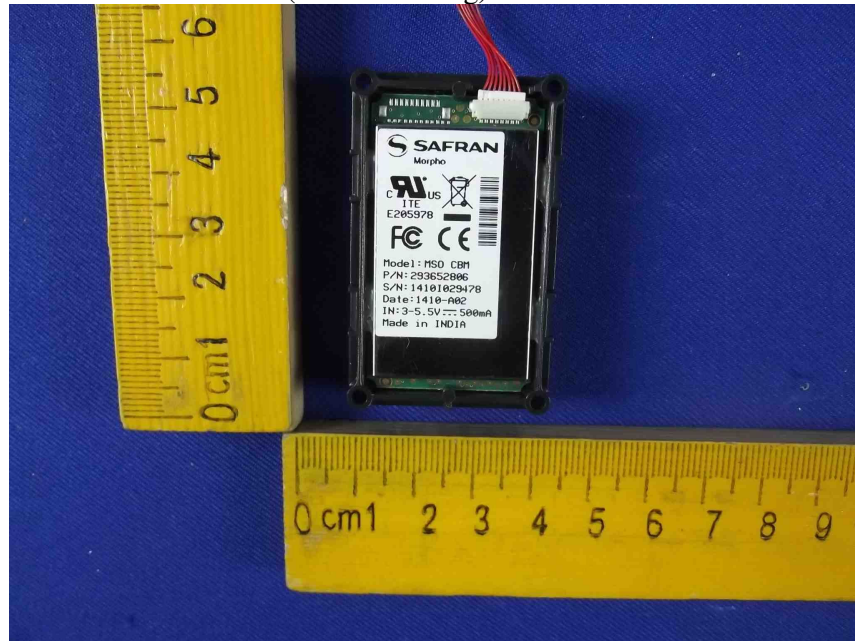
Figure 9 The EUT-Inside View (With Shielding)
