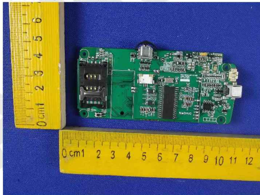
Figure 14 PCB of the EUT-Back View
