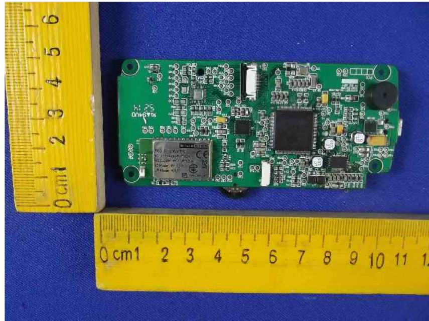
Figure 13 PCB of the EUT-Front View
