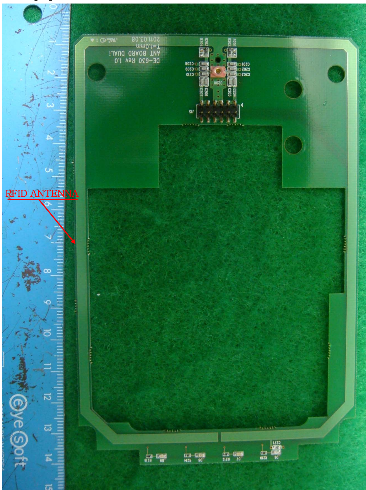
<Photograph 4: RFID antenna board - Front view>
