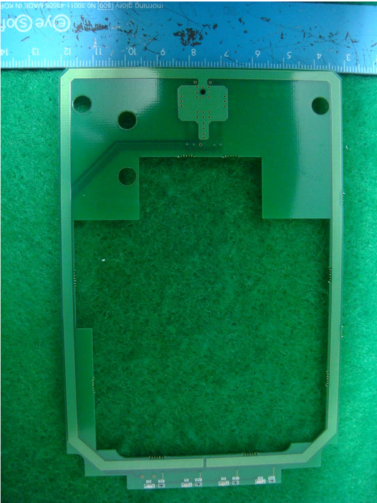
<Photograph 5: RFID antenna board - Rear view>
