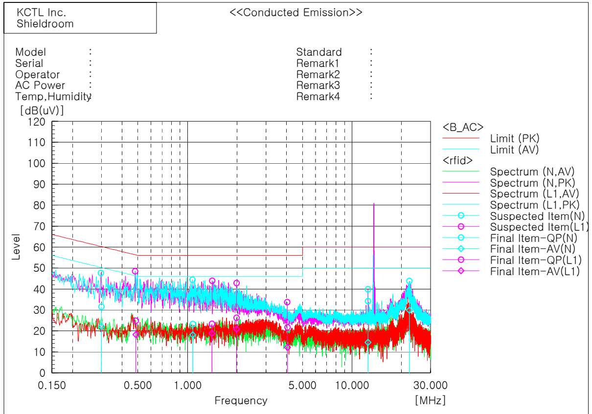
Figure4. The plot of Conducted Emission
