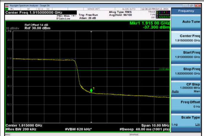
HighRange_FDD25_20MHz_1905_fullRB _High_Q16
