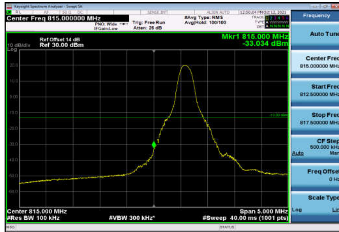
LowRange_FDD26_10MHz_820_fullRB _Low_QPSK
