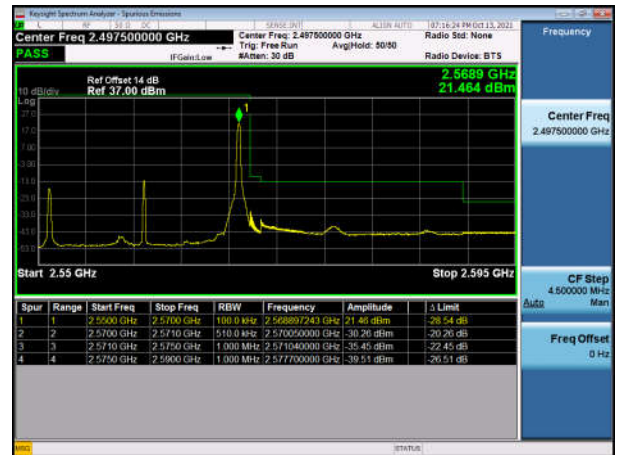
TDD7_20M High FullRB 16Q
