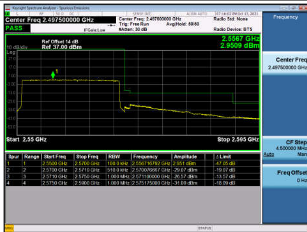
TDD7_20M High FullRB QPSK
