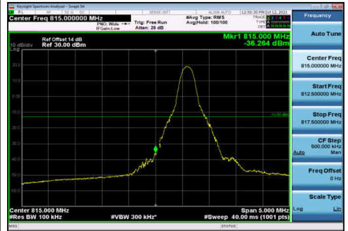
LowRange_FDD26_10MHz_820_fullRB _Low_Q16
