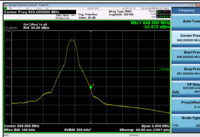
HighRange_FDD26_10MHz_844_fullRB _High_QPSK
