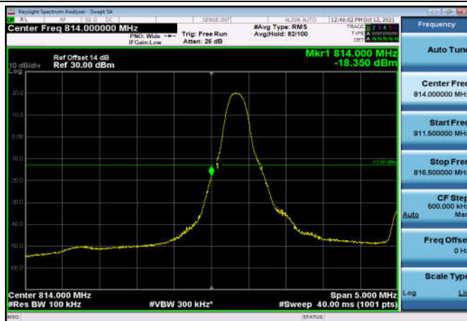
LowRange_FDD26_5MHz_816.5_fullRB _Low_QPSK
