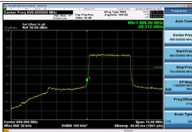
LowRange_FDD12_3MHz_700.5_fullIRB _Low_QPSK
