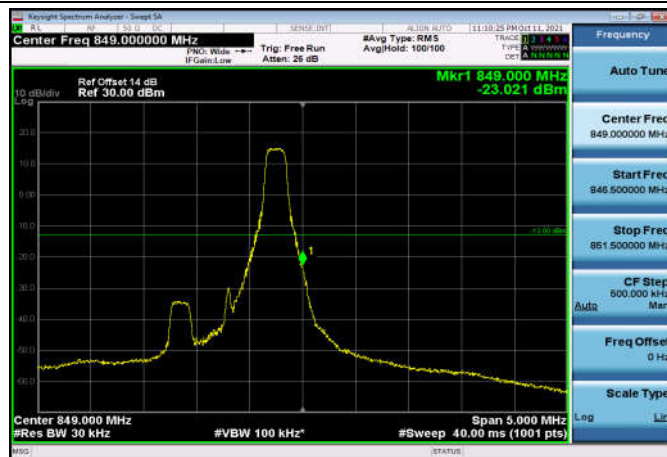
HighRange_FDD05_1.4MHz_848.3_fullRB _High_QPSK
