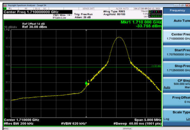
LowRange_FDD66_20MHz_1720_OneRB _low_QPSK
