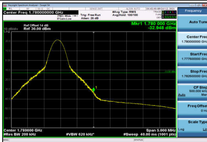
HighRange_FDD66_20MHz_1770_OneRB _high_QPSK
