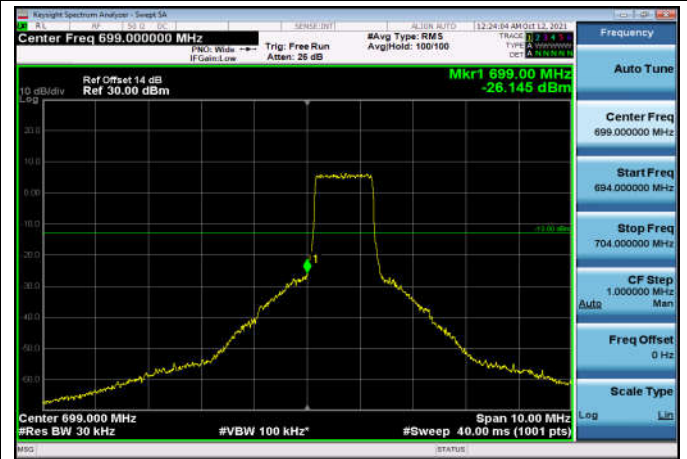
LowRange_FDD12_3MHz_700.5_OneRB _low_Q16
