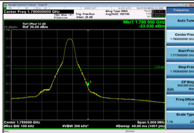
HighRange_FDD66_10MHz_1775_fullRB _High_QPSK
