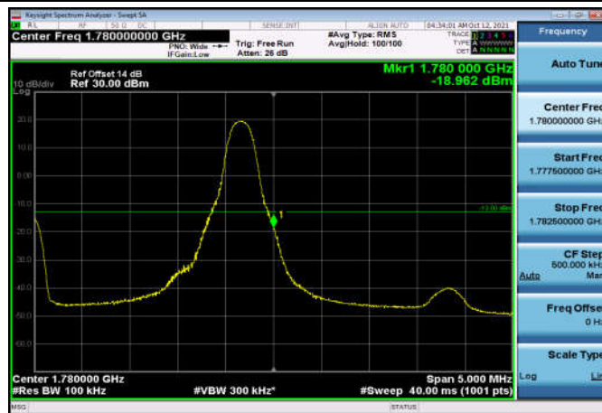
HighRange_FDD66_5MHz_1777.5_OneRB _high_QPSK
