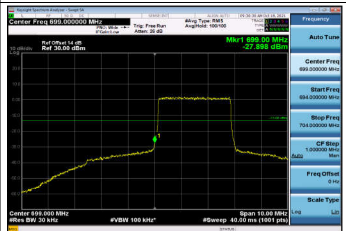
LowRange_FDD12_3MHz_700.5_fullIRB _Low_Q16
