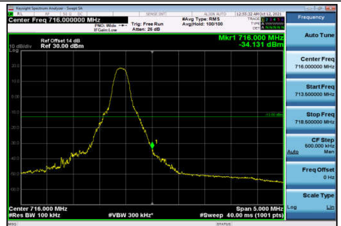
HighRange_FDD12_10MHz_711_fullRB _High_Q16
