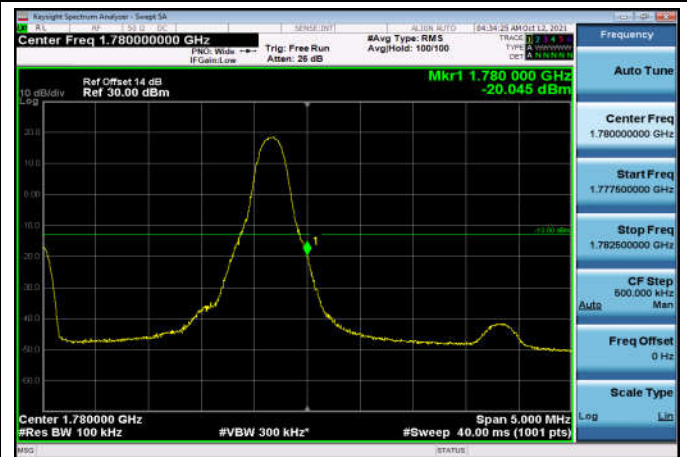
HighRange_FDD66_5MHz_1777.5_OneRB _high_Q16
