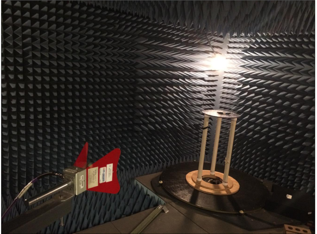
Photograph 4. Radiated Spurious Emissions, Test Setup
