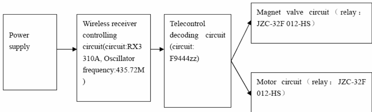
Receiver block diagram
